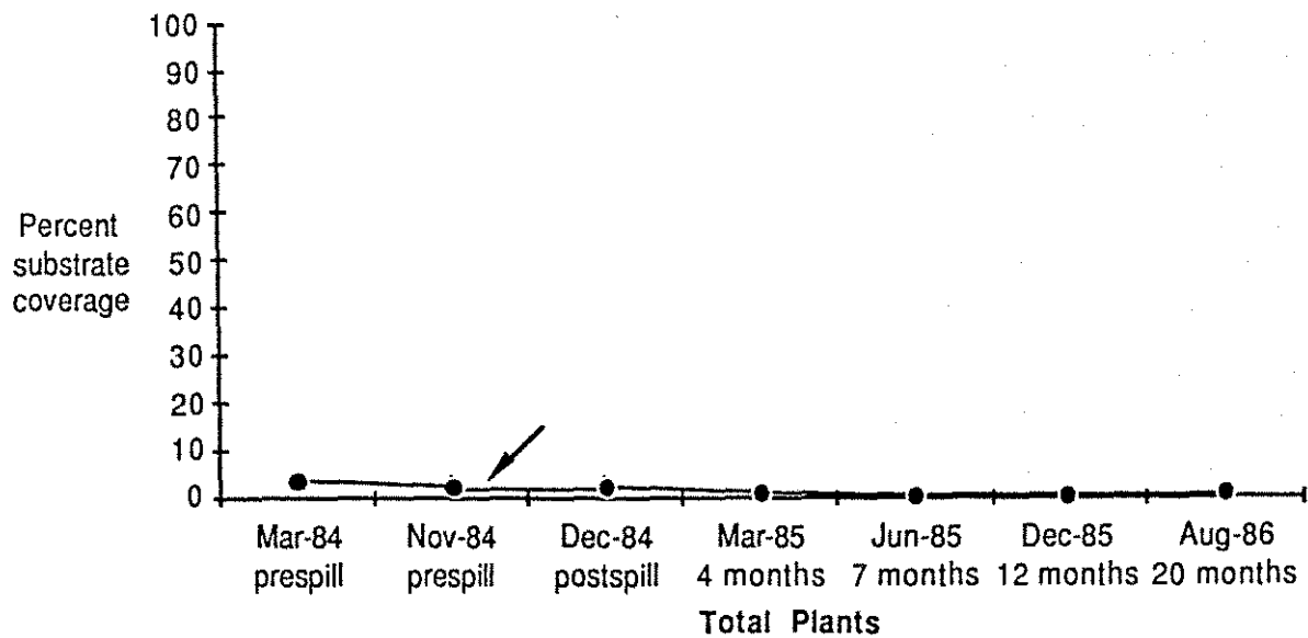
FIGURE 33. The percentage of reef substrate coverage of corals and total plants at Site D. Error bars are \pm 1 standard deviation. Arrow indicates date of site treatment.
