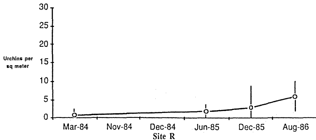
FIGURE 56. Areal densities ( \#/m^2 ) of E. lacunifer at Site D (top), Site O (middle), and Site R (bottom). Arrow indicates date of site treatment.
