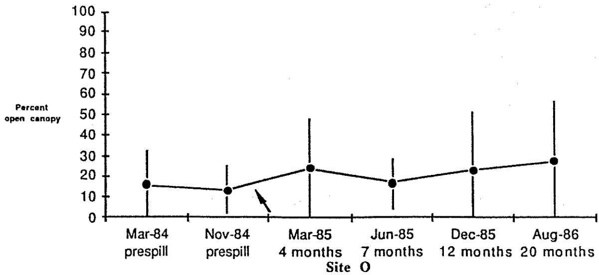
FIGURE C. Percent open canopy of the mangrove forest at Site D (top) and Site O (bottom). Arrow indicates date of spill.
