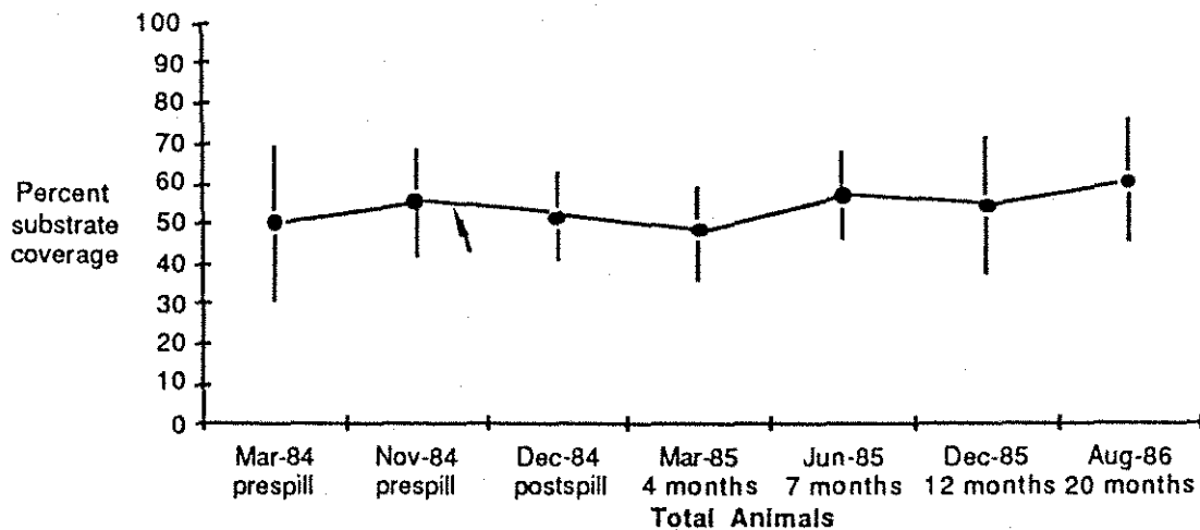
FIGURE 34. The percentage of reef substrate coverage of total organisms (top) and total animals (bottom) at Site O. Error bars are \pm 1 standard deviation. Arrow indicates date of site treatment.
