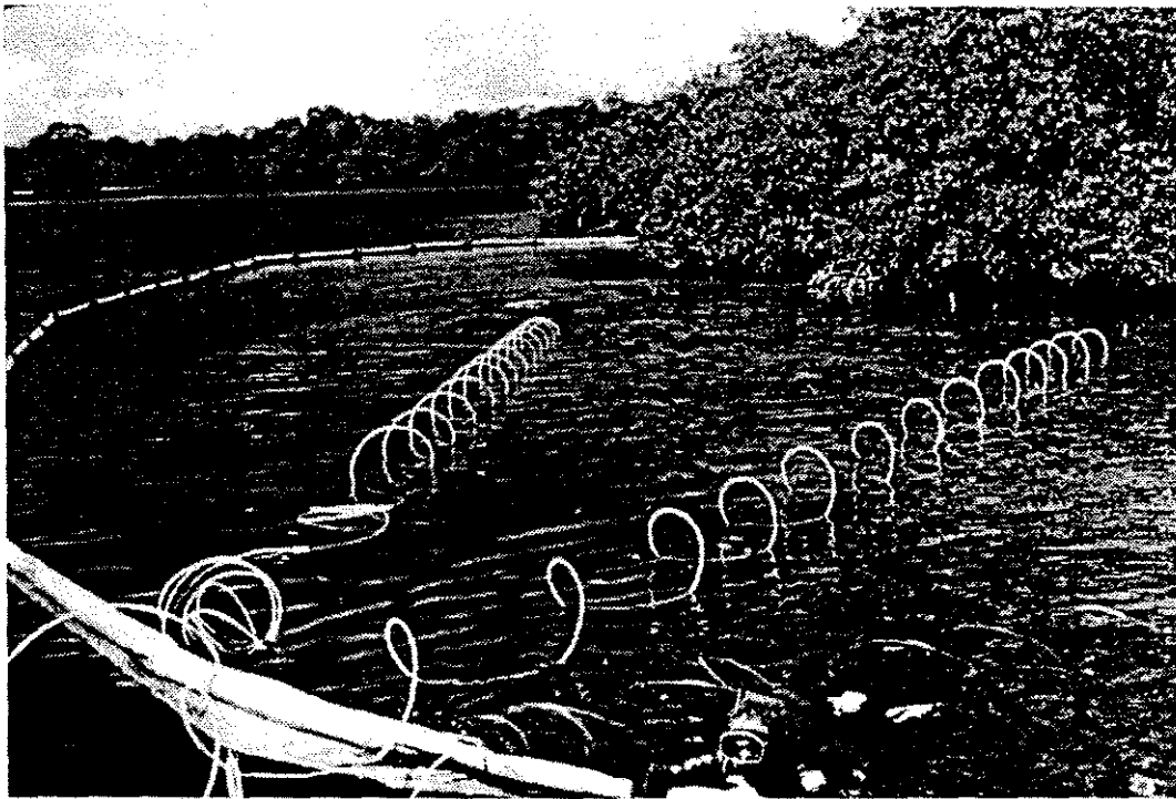
FIGURE 13. Polyethylene tubing was used to take water samples from six locations in each study site during treatment.
