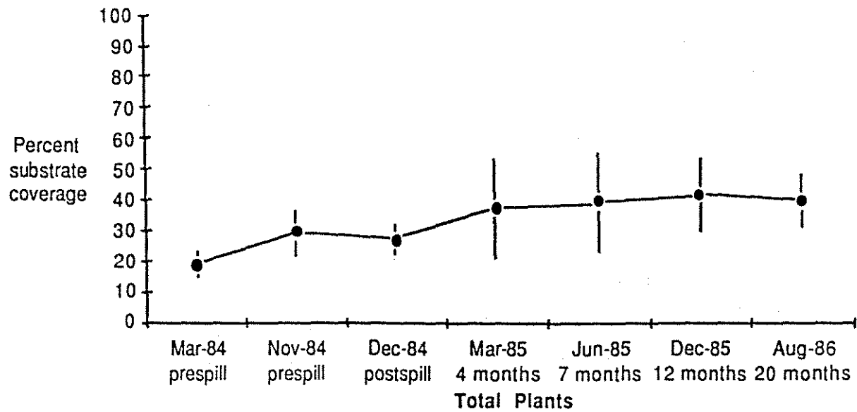
FIGURE 37. The percentage of reef substrate coverage of corals (top) and total plants (bottom) at Site R. Error bars are \pm 1 standard deviation.
