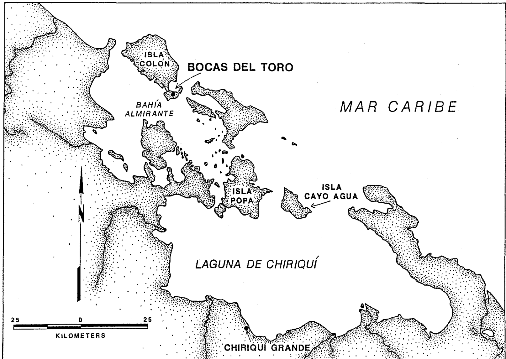
FIGURE 1. The Laguna de Chiriquí is located in northwestern Panama on the Caribbean Sea.
