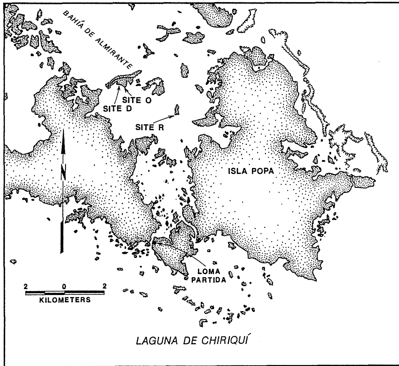
FIGURE 4. The study sites were located on a chain of islands known as the Cayos Viscayos. Sites D and O were located on Cayo Fresca, and Site R was on Cayo Ramirez.
