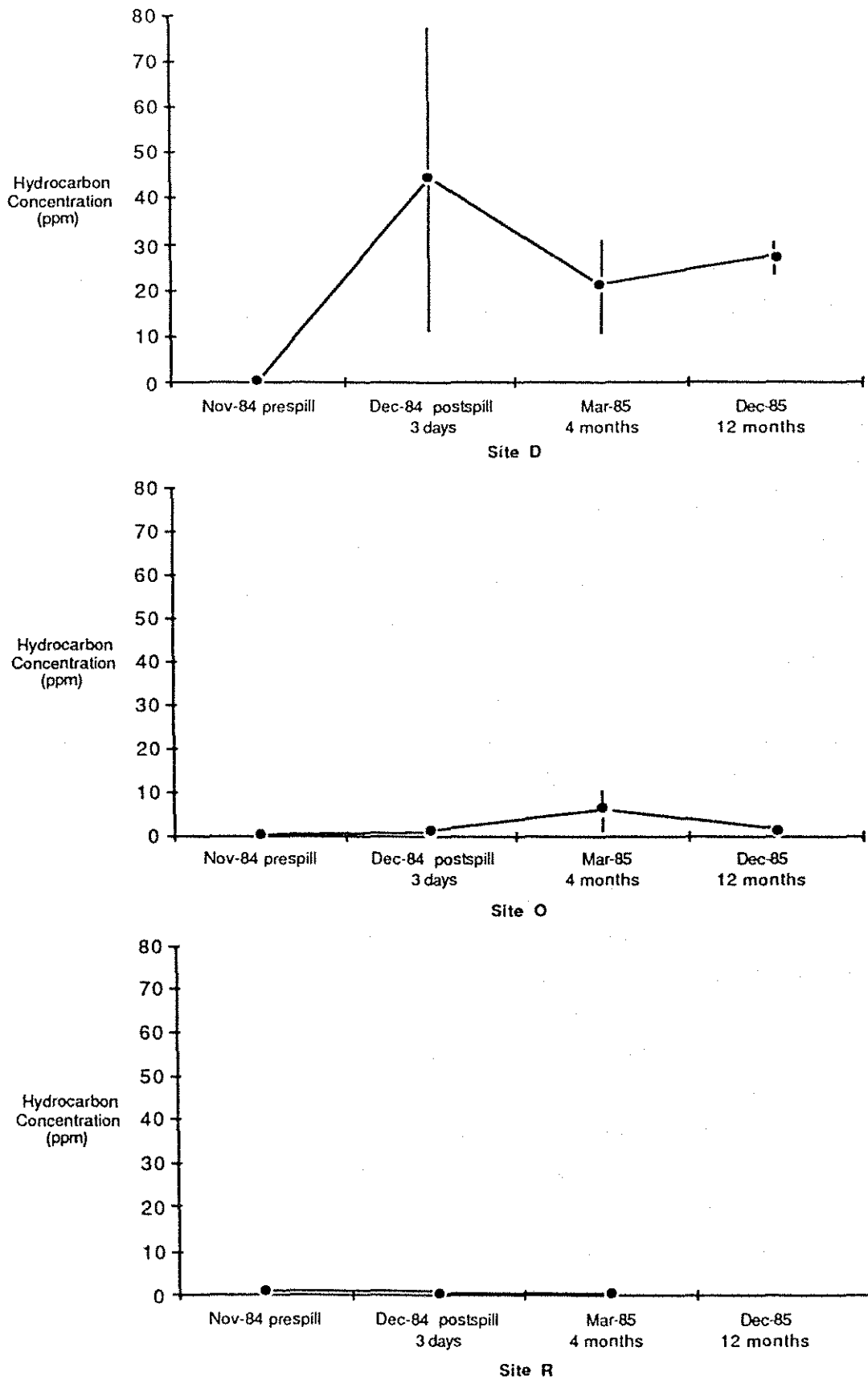
FIGURE 16. Hydrocarbon concentrations of seagrass sediments.
