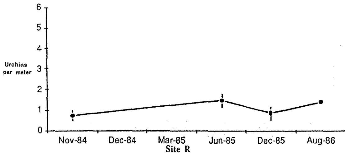
FIGURE 55. Linear densities (#/m) of Echinometra lacunter (black sea urchins) at Site D (top), Site O (middle), and Site R (bottom). Arrow indicates date of site treatment.
