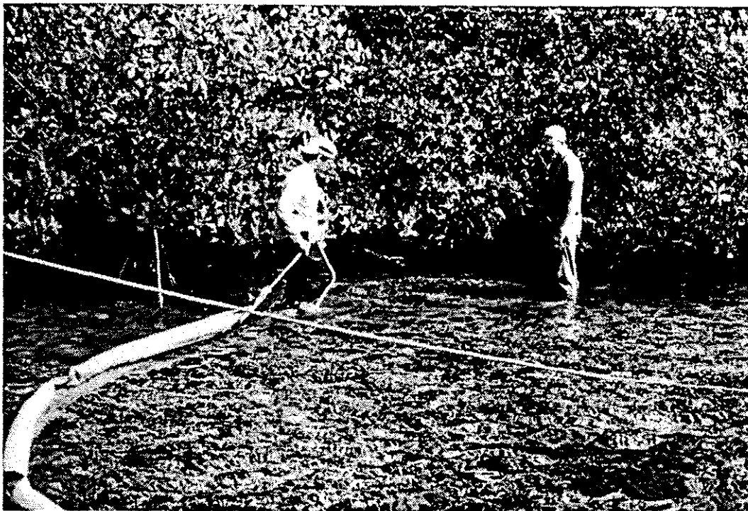
FIGURE 5. Containment booms were laid out to surround each study site. A channel was cut along the outside perimeter of the intertidal area of each site to allow the boom to be threaded through the prop roots.
