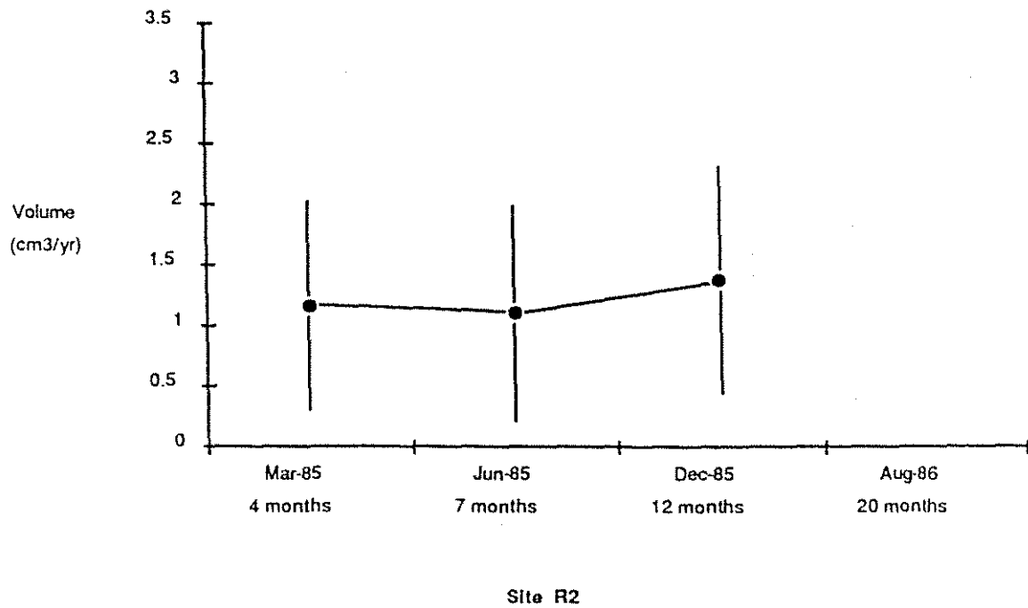
FIGURE 49. Tip volumes of P. porites specimen at Site R (top) and Site R-2 (bottom).
