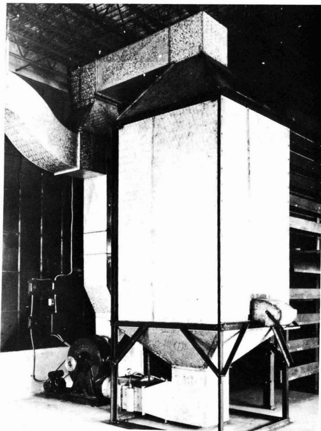
Figure 98. In-shell nut drying bin at the Hawaiian Macadamia Nut Company factory on Pohukaina Street in Honolulu in the 1930s.
