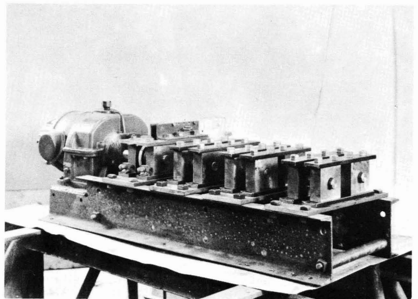
Figure 100. Probably the first nut cracker used in the industry at Honokaa Sugar Plantation to crack macadamia nuts at Honokaa in the 1930s. This machine was designed and built by Otto Hermann.
