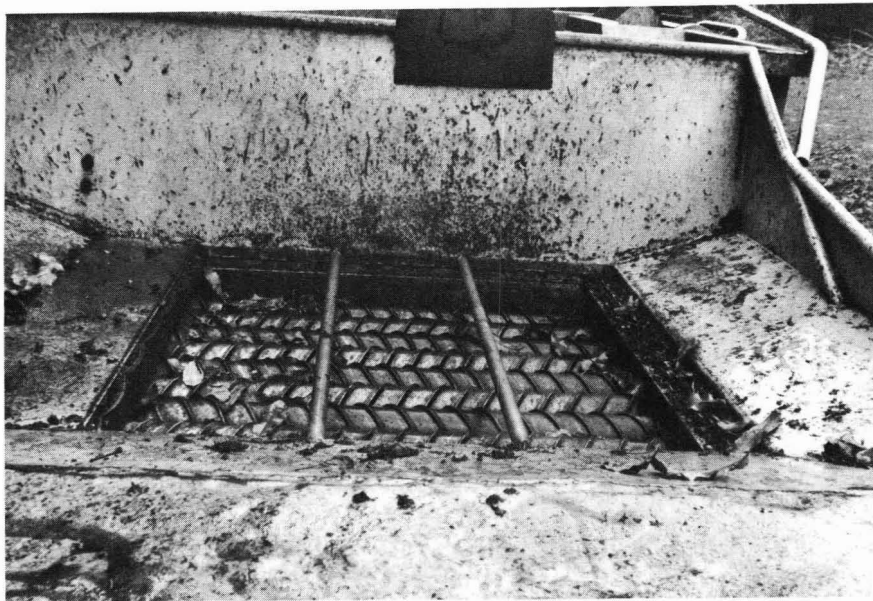
Figure 84. Leaf stripper showing the counter-rotating scrolls to separate the nuts from the leaves.
