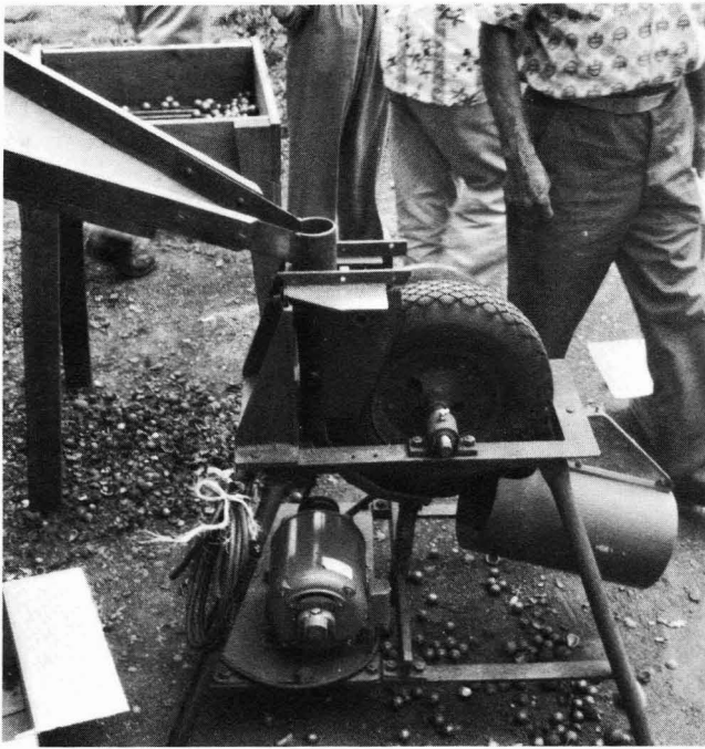
Figure 126. Made by a grower in the Kohala area, this portable nut husker uses a small wheelbarrow tire.
