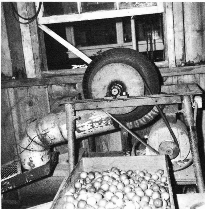
Figure 87. Rubber-tire husker with its power source an electric motor, still used by Francis Takahashi on Kauai.
