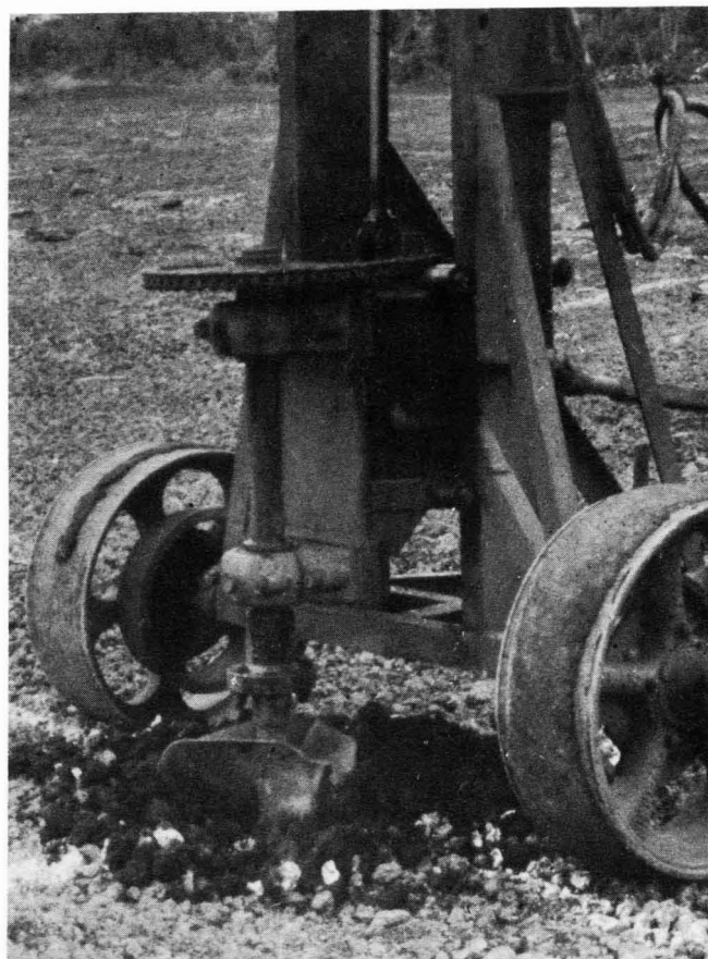
Figure 58. The original posthole digger fabricated by Stubenberg and Company in Hilo for use at Keau Orchard in the early 1950s. Note the wide auger especially designed for macadamia on aa lava land. This unit derived its power from the power takeoff on a tractor. In recent years, a backhoe has been used to further reduce cost.
