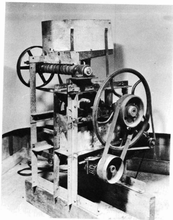
Figure 97. A macadamia nut husker developed by W. P. Naquin and Otto Hermann and used in the industry at the Honokaa Sugar Plantation in the late 1930s.
