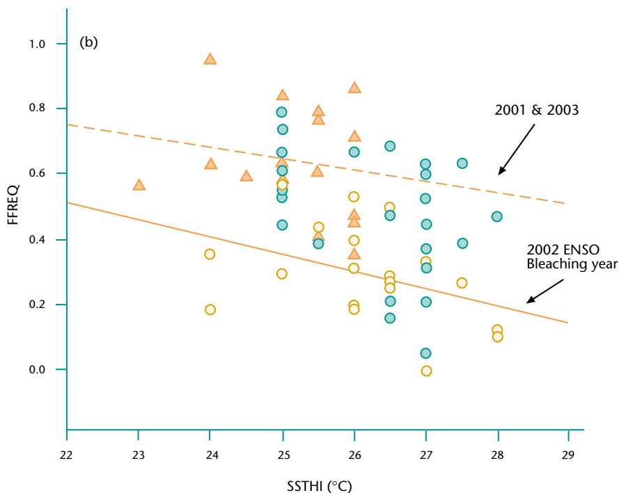
Figure 14.10 Puffinus pacificus : the effect of sea surface temperature at Heron Island (SST HI ) on: feeding frequency ( F_{\text{FREQ}} ) in 2001 (▲), 2002 (○) and 2003 (●). There was a significant effect of SST HI on F_{\text{FREQ}} across years ( F_{\text{FREQ}} = 2.856 - 0.092 \text{ SST}_{\text{HI}} ). The effect of year on F_{\text{FREQ}} was also significant. There was no effect of year on SST HI . The dashed line represents the 2001–2003 regressions while the 2002 regression is represented by the solid line 92
