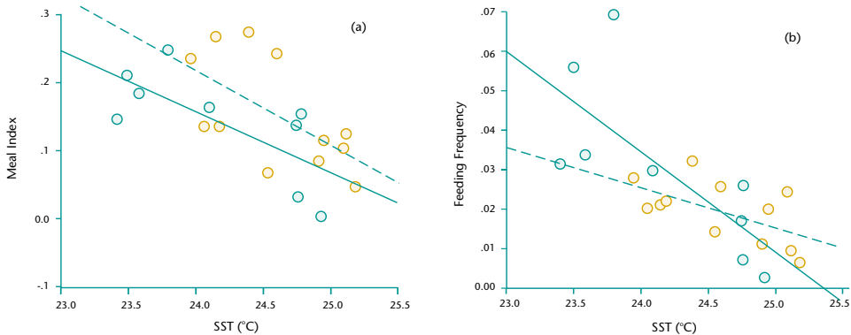
Figure 14.6 Sterna fuscata : effect of daily sea surface temperature (SST) at Michaelmas Cay on (a) age-adjusted Meal Index (○), 15 September to 3 October) of 2004 and (○), 20 May to 22 June) of 2005 and on (b) age-adjusted feeding frequency during the same periods in 2004 (○) and 2005 (○) 37
