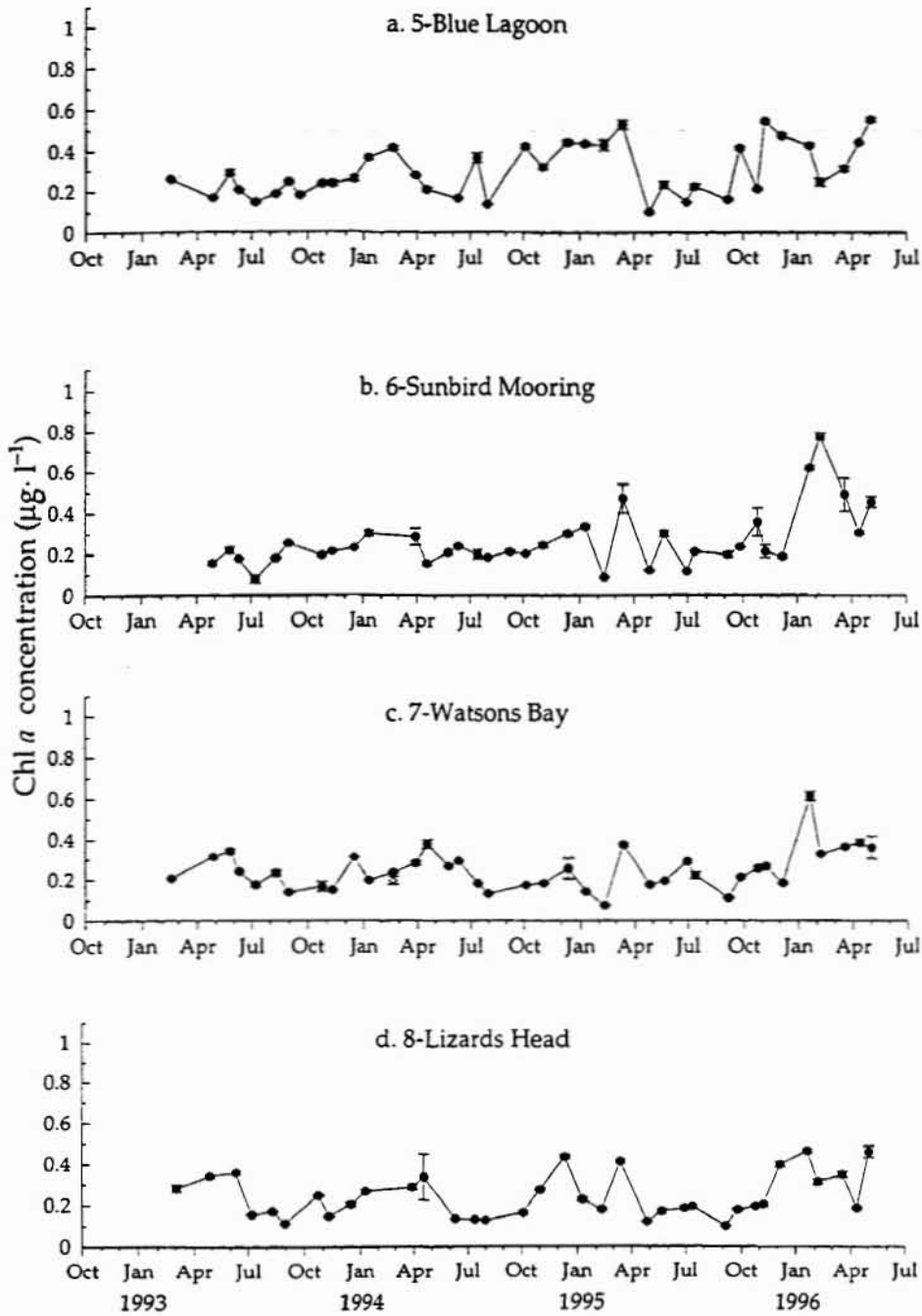
Figure 5.8 Lizard stations 5–8: mean ( \pm 1 S.E.) monthly near-surface (●) and near-bottom (○) chlorophyll a concentrations ( \mu\text{g L}^{-1} )
