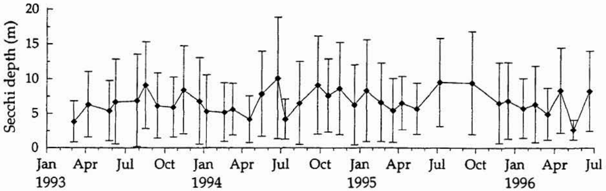
Figure 9.4 Keppel Bay: mean ( \pm 1 S.D.) monthly Secchi depth (metres)
