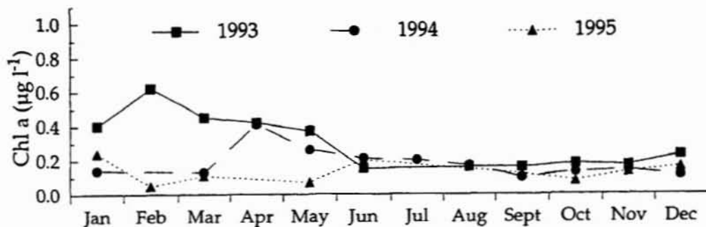
Figure 7.8 Offshore Cairns stations: median monthly chlorophyll a concentrations ( \mu\text{g L}^{-1} ) in 1993–95
