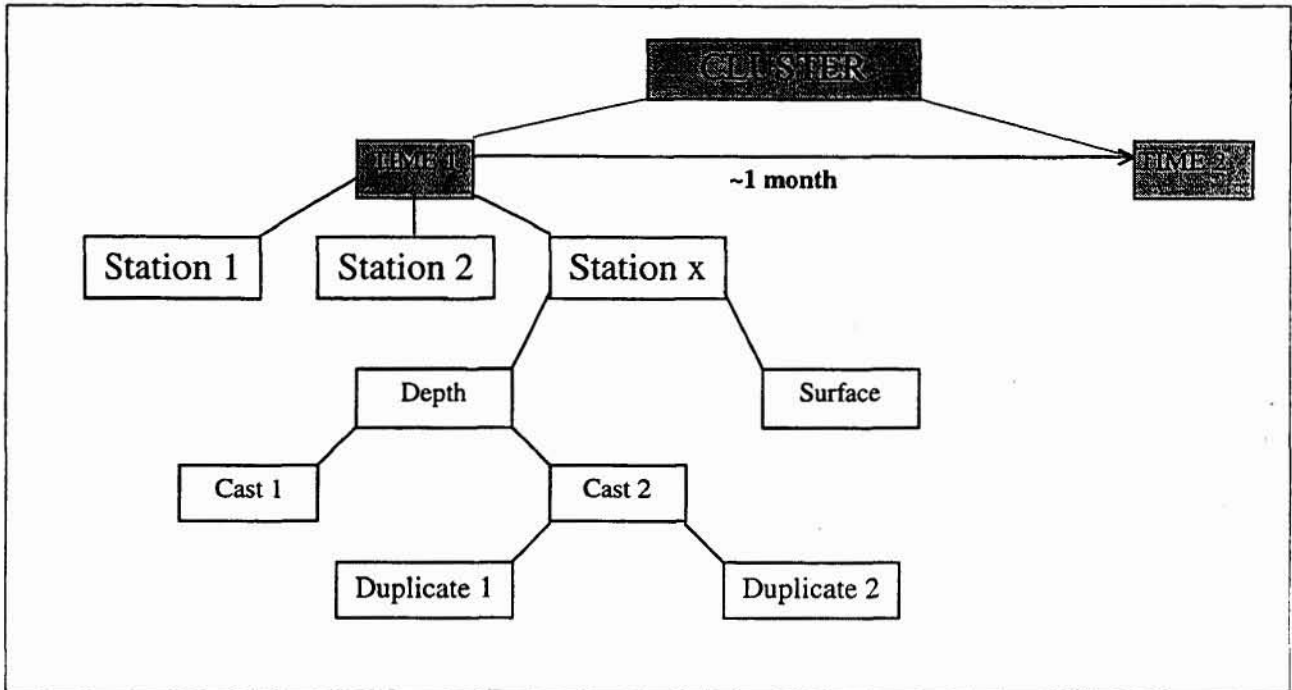
Figure 4.1 Schematic of chlorophyll a sampling strategy within each cluster
