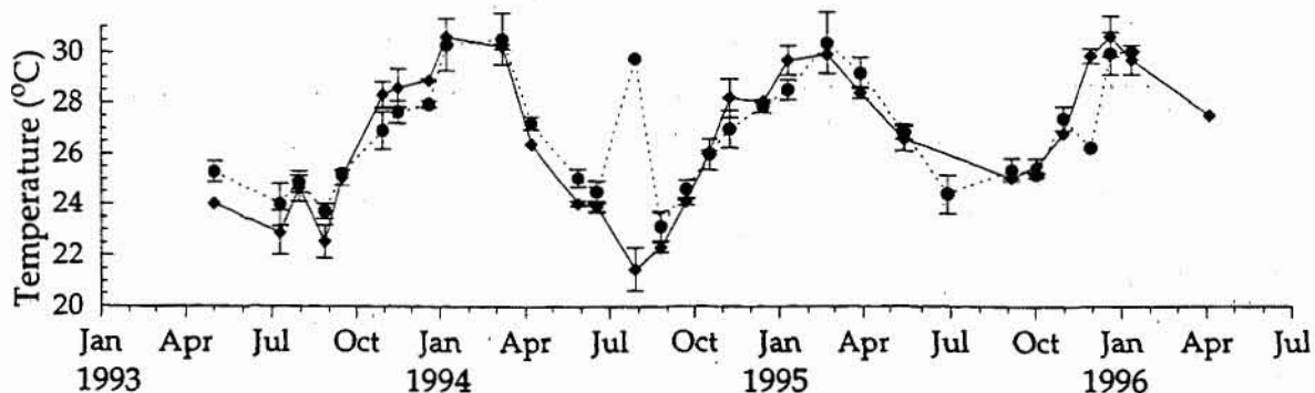
Figure 7.1 Cairns: mean ( \pm 1 S.D.) monthly surface temperature ( ^{\circ}\text{C} ) at inshore ( \blacklozenge ) and offshore ( \bullet ) stations
