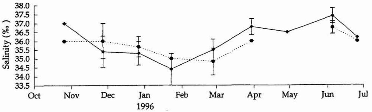
Figure 8.3 Townsville: mean ( \pm 1 S.D.) monthly surface salinity (‰) at inshore (◆) and offshore (●) stations
