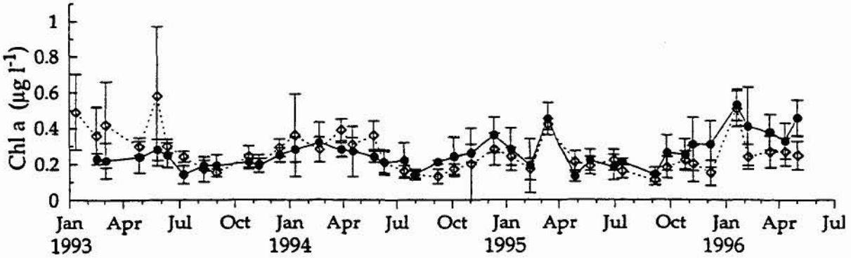
Figure 5.5 Lizard : mean ( \pm 1 S.D.) monthly surface chlorophyll a concentration ( \mu\text{g L}^{-1} ) at stations 1–4 (○) and 5–8 (●)
