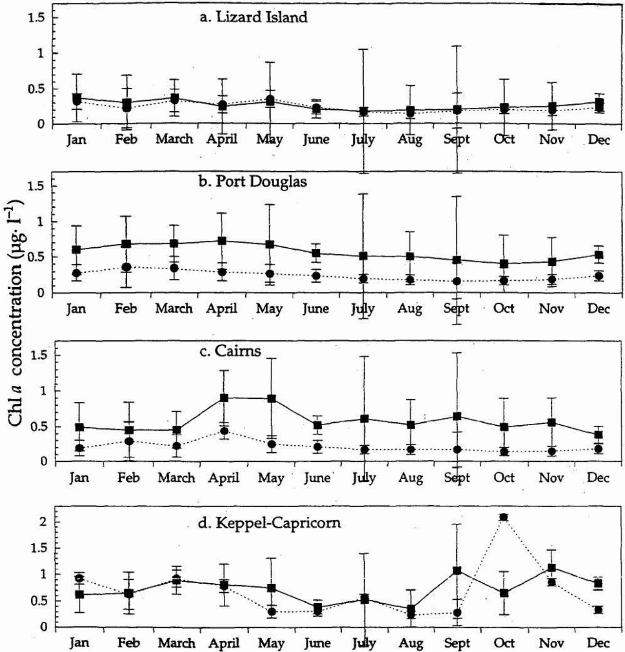
Figure 10.3 Regional monthly mean ( \pm 1 S.D.) chlorophyll a concentration ( \mu\text{g L}^{-1} ) aggregated over years. Data are grouped into inshore(■) and offshore(●) clusters
