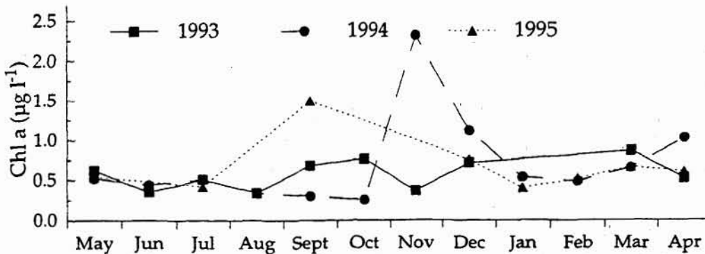
Figure 9.6 Keppel Bay: median monthly chlorophyll a concentrations ( \mu\text{g L}^{-1} ) in 1993–95
