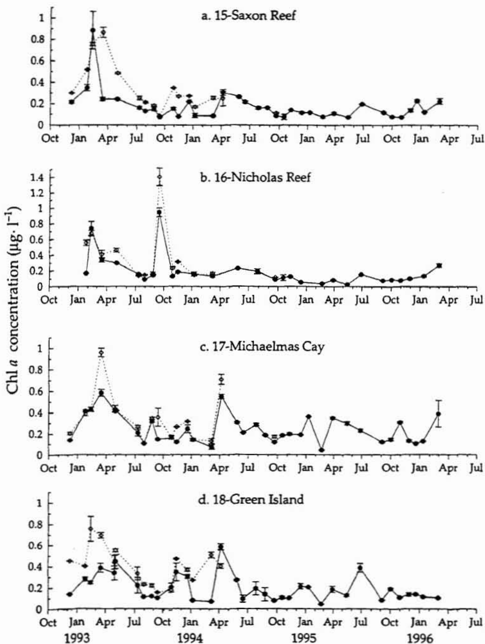
Figure 7.9 Offshore Cairns stations: mean ( \pm 1 S.E.) monthly near-surface ( \bullet ) and near-bottom ( \diamond ) chlorophyll a concentrations ( \mu\text{g L}^{-1} )
