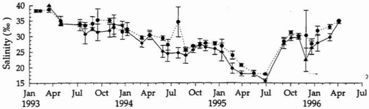
Figure 7.3 Cairns: mean ( \pm 1 S.D.) monthly surface salinity (‰) at inshore ( \blacklozenge ) and offshore ( \bullet ) stations
