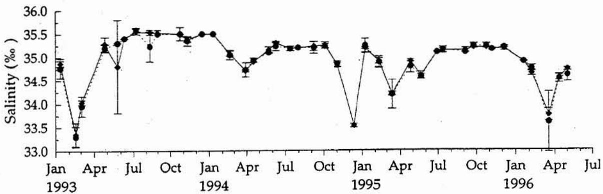
Figure 5.3 Lizard: mean ( \pm 1 S.D.) monthly surface salinity (‰) at stations 5–8 around Lizard Island (◆) and stations 1–4 (●)
