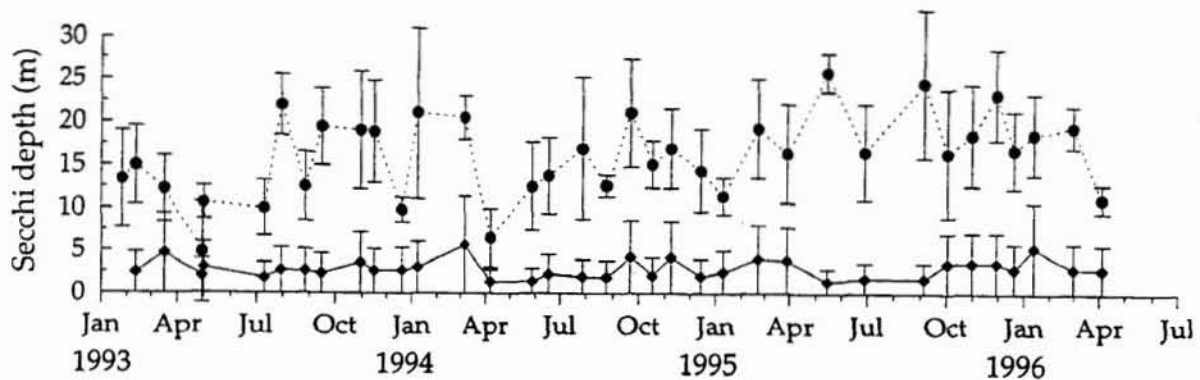
Figure 7.4 Cairns: mean ( \pm 1 S.D.) monthly Secchi depth (metres) at inshore ( \blacklozenge ) and offshore ( \bullet ) stations
