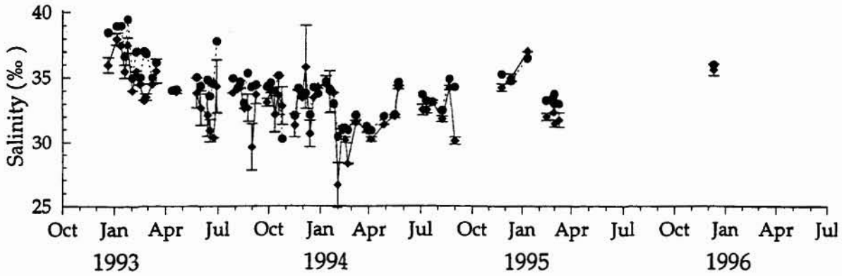
Figure 6.3 Port Douglas: mean ( \pm 1 S.D.) monthly surface salinity (‰) at inshore ( \blacklozenge ) and offshore ( \bullet ) stations
