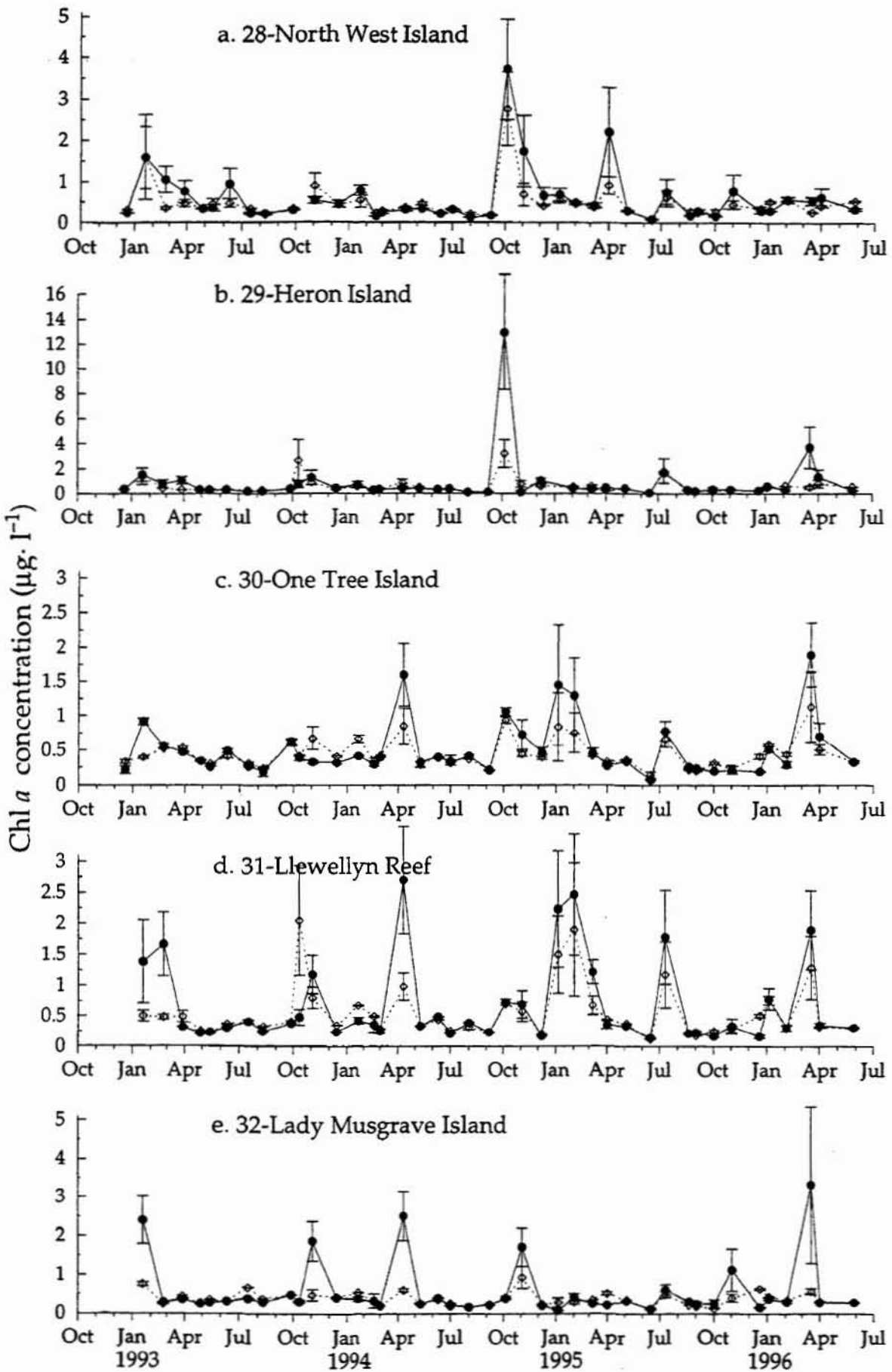
Figure 9.14 Capricorn: mean ( \pm 1 S.E.) monthly near-surface (●) and near-bottom (◊) chlorophyll a concentrations ( \mu\text{g L}^{-1} )
