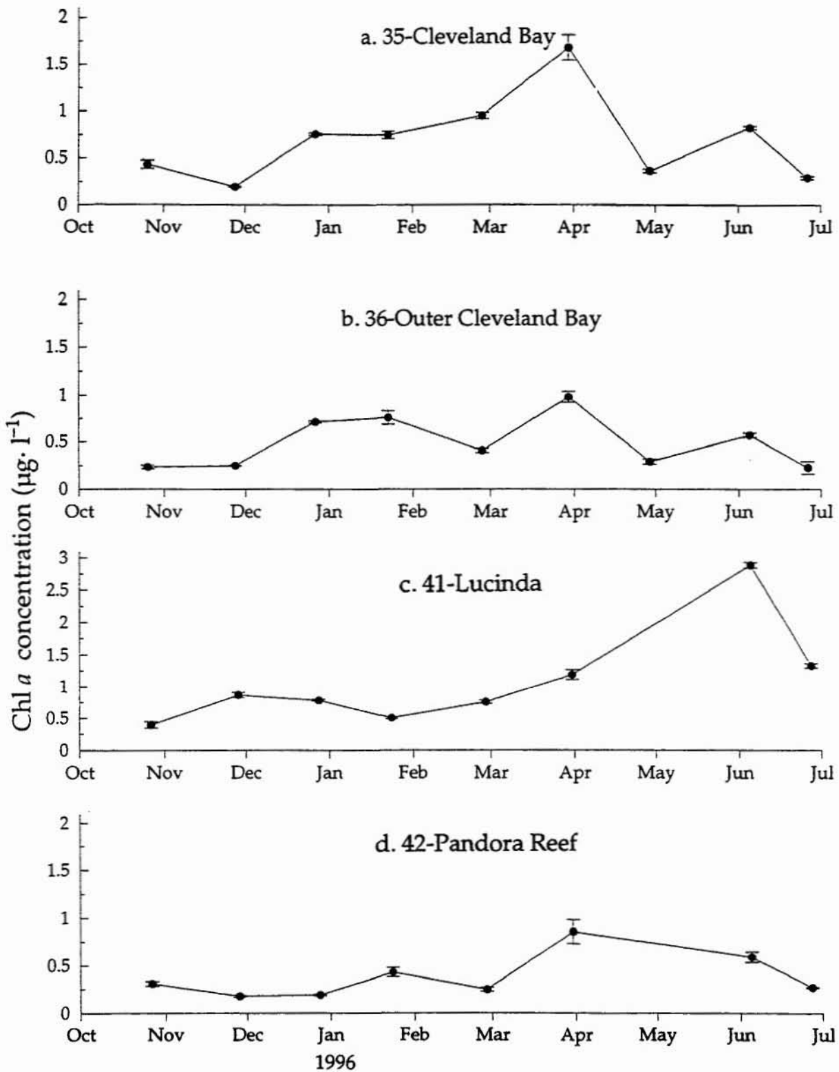
Figure 8.6 Inshore Townsville stations: mean ( \pm 1 S.E.) monthly near-surface chlorophyll a concentrations ( \mu\text{g L}^{-1} )
