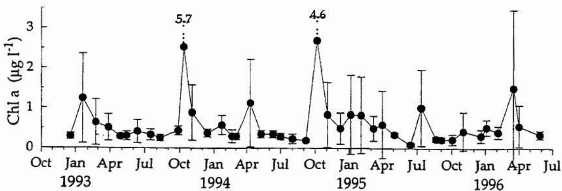
Figure 9.12 Capricorn: mean ( \pm 1 S.E.) monthly surface chlorophyll a concentration ( \mu\text{g L}^{-1} )
