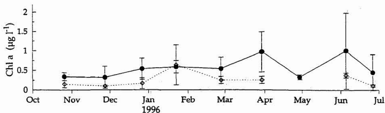
Figure 8.5. Townsville: mean ( \pm 1 S.D.) monthly surface chlorophyll a concentration ( \mu\text{g L}^{-1} ) at inshore (●) and offshore (◊) stations
