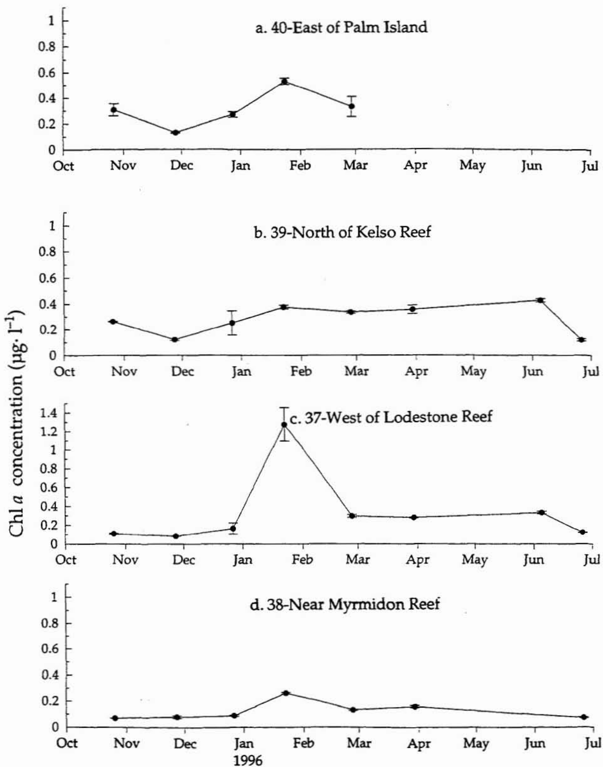
Figure 8.7 Offshore Townsville stations: mean ( \pm 1 S.E.) monthly near-surface chlorophyll a concentrations ( \mu\text{g}\cdot\text{L}^{-1} )
