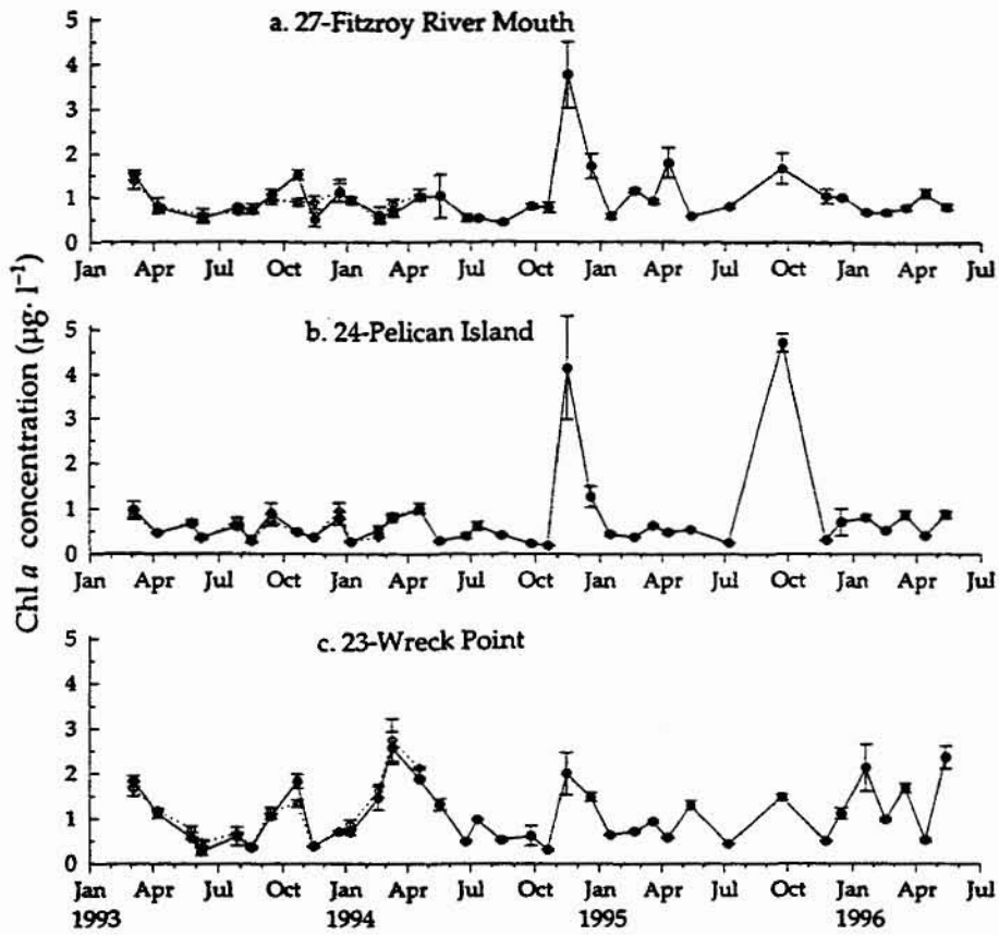
Figure 9.7 Keppel Bay: mean ( \pm 1 S.E.) monthly near-surface ( \bullet ) and near-bottom ( \diamond ) chlorophyll a concentrations ( \mu\text{g}\cdot\text{L}^{-1} ) at stations 23, 24 and 27
