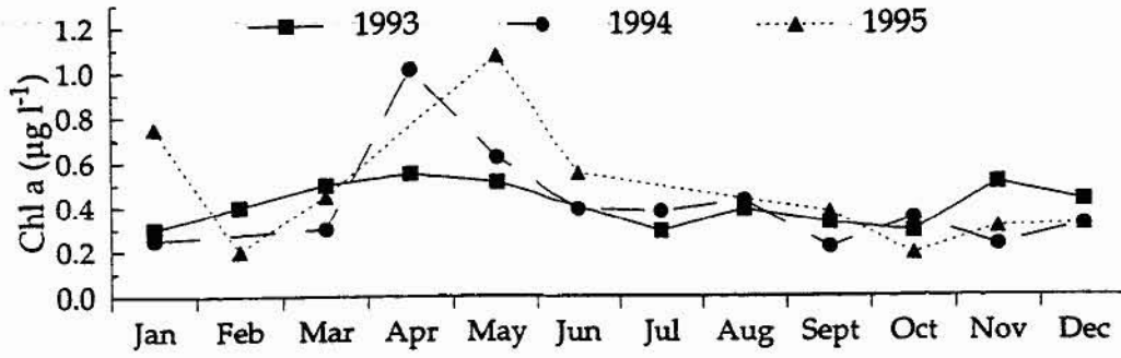
Figure 7.6 Inshore Cairns stations: median monthly chlorophyll a concentrations ( \mu\text{g}\cdot\text{L}^{-1} ) in 1993–95
