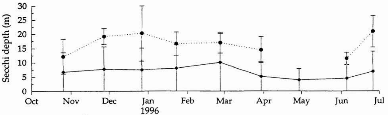
Figure 8.4 Townsville: mean ( \pm 1 S.D.) monthly Secchi depth (metres) at inshore (◆) and offshore (●) stations
