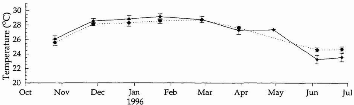
Figure 8.1 Townsville: mean ( \pm 1 S.D.) monthly surface temperature ( ^{\circ}\text{C} ) at inshore ( \blacklozenge ) and offshore ( \bullet ) stations
