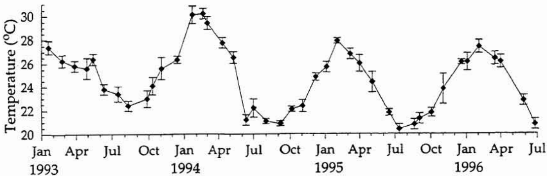
Figure 9.9 Capricorn: mean ( \pm 1 S.D.) monthly surface temperature (°C)
