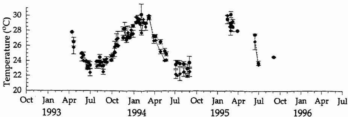
Figure 6.1 Port Douglas: mean ( \pm 1 S.D.) monthly surface temperature ( ^{\circ} C) at inshore ( \blacklozenge ) and offshore ( \bullet ) stations
