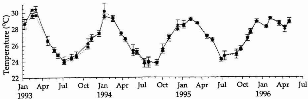
Figure 5.1 Lizard : mean ( \pm 1 S.D.) monthly surface temperature ( ^{\circ}\text{C} ) at stations 5–8 around Lizard Island ( \blacklozenge ) and stations 1–4 ( \bullet )
