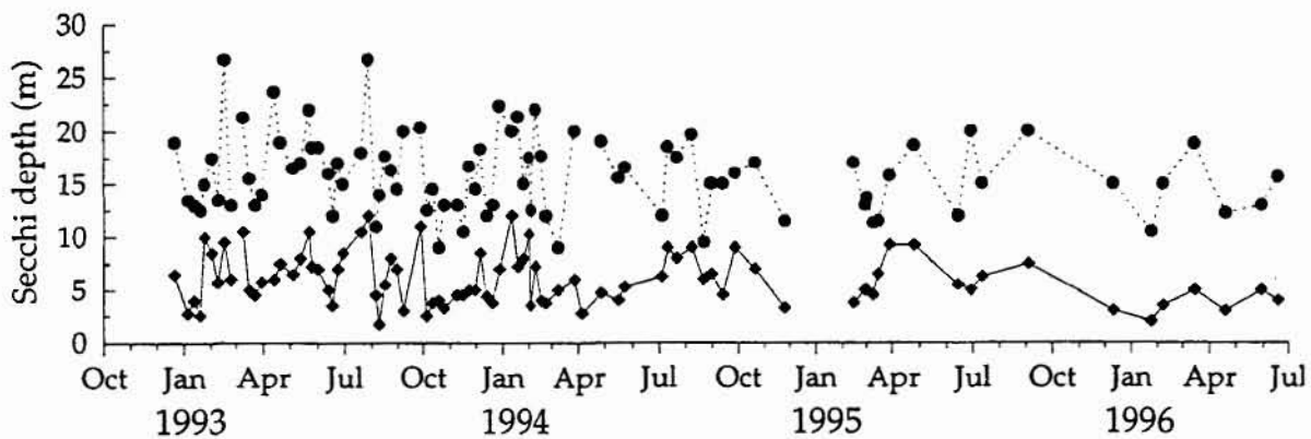
Figure 6.4 Port Douglas: mean monthly Secchi depth (metres) at inshore ( \blacklozenge ) and offshore ( \bullet ) stations. Error bars omitted for clarity.
