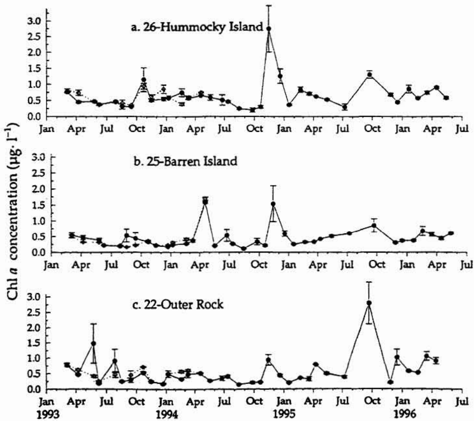
Figure 9.8 Keppel Bay: mean ( \pm 1 S.E.) monthly near-surface ( \bullet ) and near-bottom ( \diamond ) chlorophyll a concentrations ( \mu\text{g}\cdot\text{L}^{-1} ) at stations 22, 25 and 26
