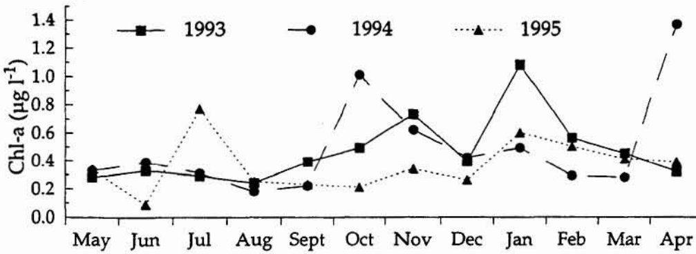
Figure 9.13 Capricorn: median monthly chlorophyll a concentrations ( \mu\text{g L}^{-1} ) in 1993–95
