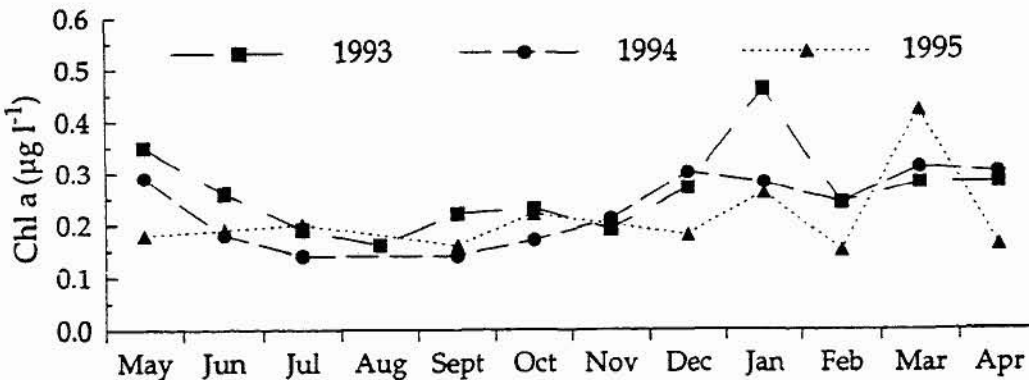
Figure 5.6 Lizard : median monthly chlorophyll a concentrations ( \mu\text{g L}^{-1} ) averaged over stations 1–8 in 1993–95
