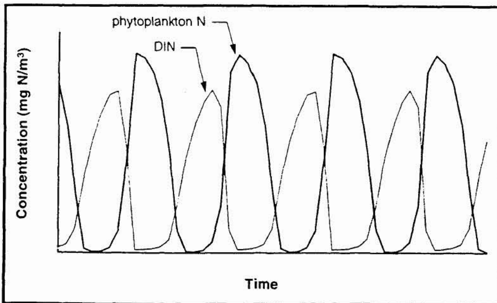
Figure 2.2 Example of NPZ models, from Harris et al. (1996): (a) plot of concentration of DIN and phytoplankton N vs time, in response to a constant load exceeding the threshold load by 20%; (b) change in mean and maximum phytoplankton biomass in response to different nutrient loads
