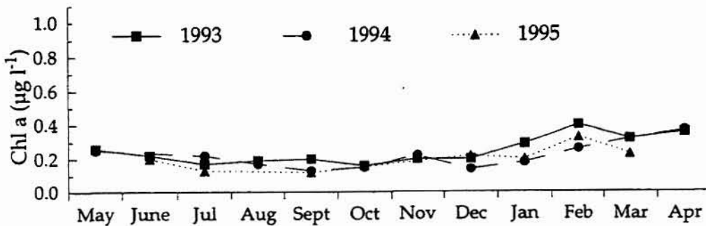
Figure 6.8 Offshore Port Douglas: median monthly chlorophyll a concentrations ( \mu\text{g L}^{-1} ) in 1993–95
