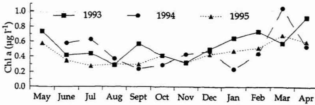
Figure 6.6 Inshore Port Douglas stations: median monthly chlorophyll a concentrations ( \mu\text{g L}^{-1} ) in 1993–95
