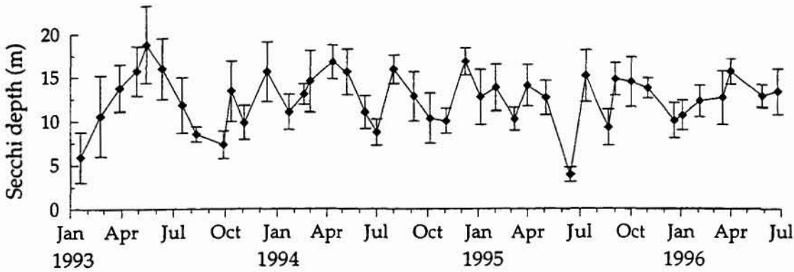
Figure 9.11 Capricorn: mean ( \pm 1 S.D.) monthly Secchi depth (metres)
