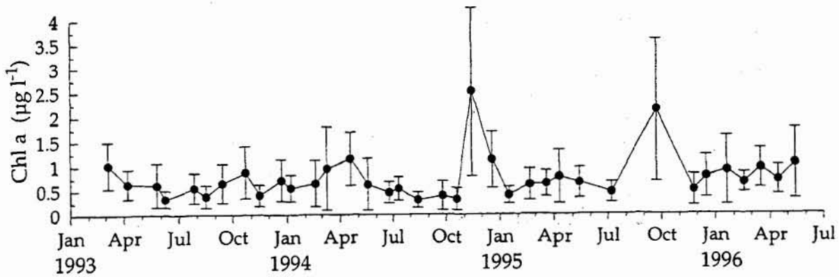
Figure 9.5 Keppel Bay: mean ( \pm 1 S.D.) monthly surface chlorophyll a concentration ( \mu\text{g L}^{-1} )
