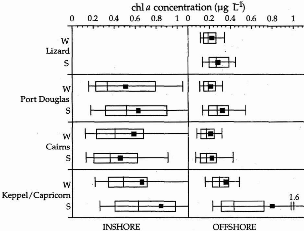
Figure 10.1 Box plots of surface chlorophyll a concentrations ( \mu\text{g L}^{-1} ) grouped by region, cross-shelf position (inshore, offshore) and season (summer [S], winter [W]). Box plots represent the spread of data. The box contains the middle half (50%) of the data, the outer and inner lines representing the 75th and 25th percentiles respectively. The line inside the box is the median (50th percentile). The whiskers extending from either end of the box encompass the data within the 10th and 90th percentile. The ■ represents the arithmetic mean of the data.
