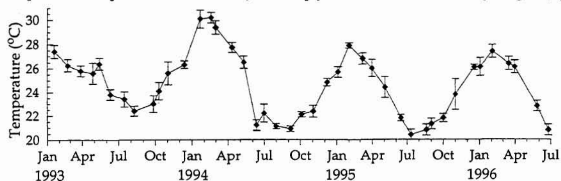
Figure 9.1 Keppel Bay: mean ( \pm 1 S.D.) monthly surface temperature ( ^{\circ} C)
