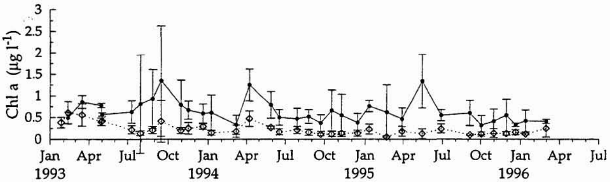
Figure 7.5 Cairns: mean ( \pm 1 S.D.) monthly surface chlorophyll concentration ( \mu\text{g L}^{-1} ) at inshore ( \diamond ) and offshore ( \bullet ) stations
