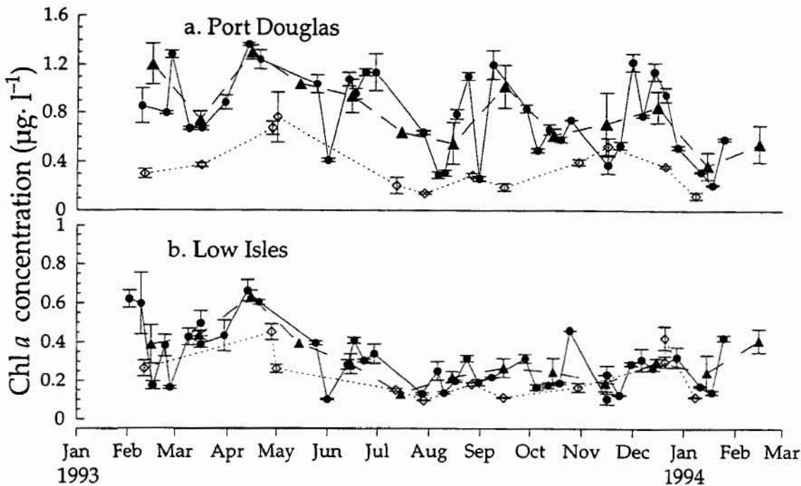
Figure 10.4 Comparison of mean ( \pm 1 S.E.) chlorophyll a concentrations ( \mu\text{g L}^{-1} ) recorded at stations 10 and 20 (a) and stations 11 and 21 (b) over different sampling frequencies: (●) samples collected weekly at 10 and 11; (▲) monthly (calendar) average of samples collected weekly at stations 10 and 11; (◇). Monthly samples collected at stations 20 and 21.
