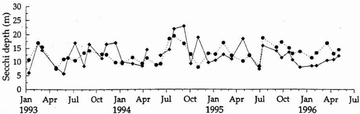
Figure 5.4 Lizard: mean monthly Secchi depth (metres) at stations 5–8 around Lizard Island (◆) and stations 1–4 (●). Error bars omitted for clarity.
