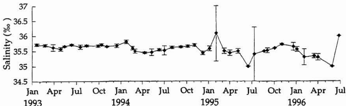
Figure 9.10 Capricorn: mean ( \pm 1 S.D.) monthly surface salinity (‰)
