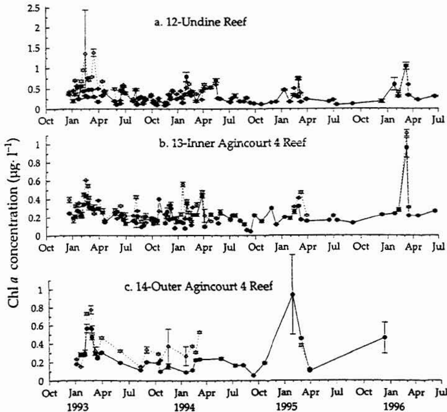
Figure 6.9 Offshore Port Douglas stations: mean ( \pm 1 S.E.) monthly near-surface ( \bullet ) and near-bottom ( \circ ) chlorophyll a concentrations ( \mu\text{g L}^{-1} )
