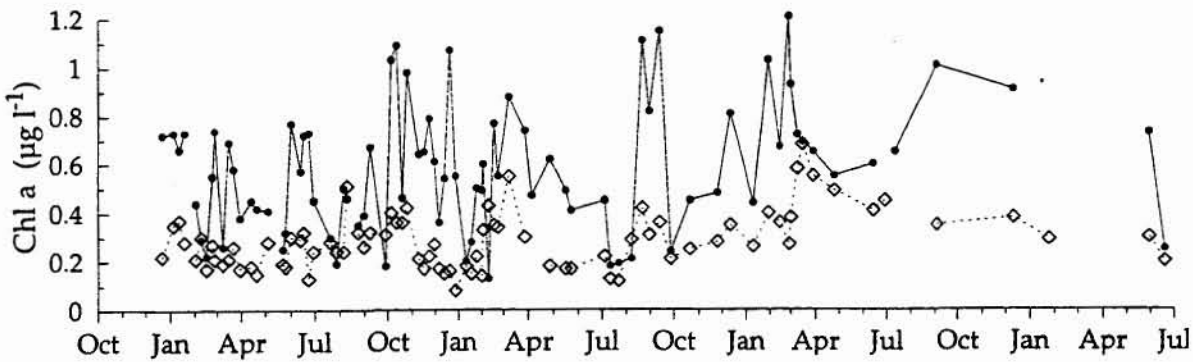
Figure 6.5 Port Douglas: mean monthly surface chlorophyll a concentration (µg L -1 ) at inshore (●) and offshore (◊) stations. Error bars omitted for clarity.
