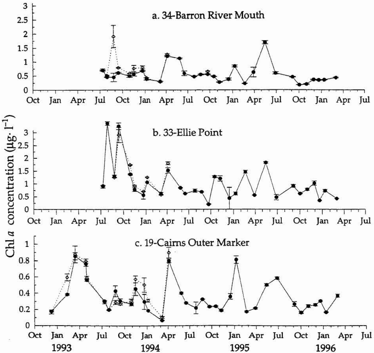
Figure 7.7 Inshore Cairns stations: Mean monthly ( \pm 1 S.E.) near-surface ( \bullet ) and near-bottom ( \diamond ) chlorophyll a concentrations ( \mu\text{g}\cdot\text{L}^{-1} )
