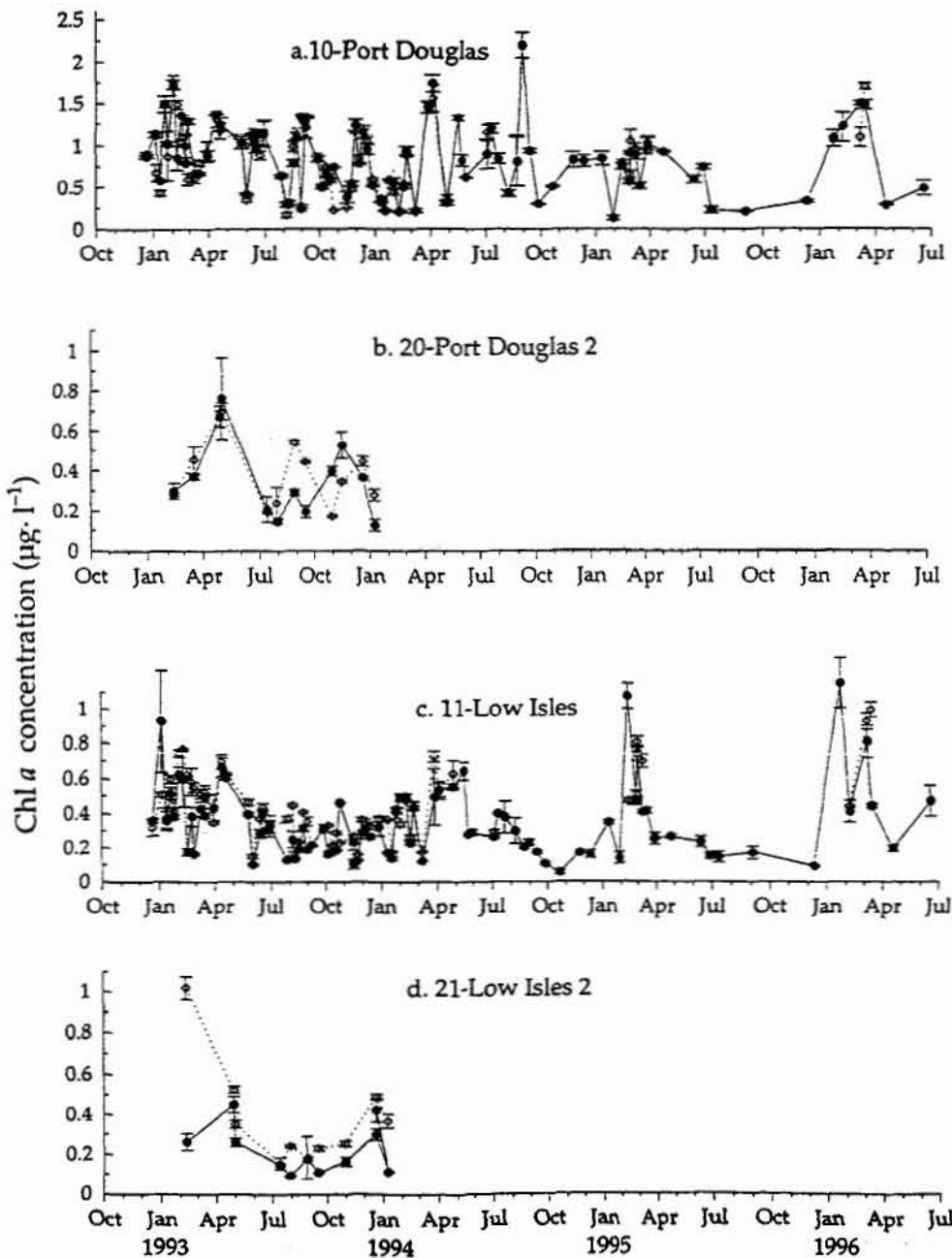
Figure 6.7 Inshore Port Douglas stations: mean ( \pm 1 S.E.) monthly near-surface (●) and near-bottom (◊) chlorophyll a concentrations ( \mu\text{g L}^{-1} )
