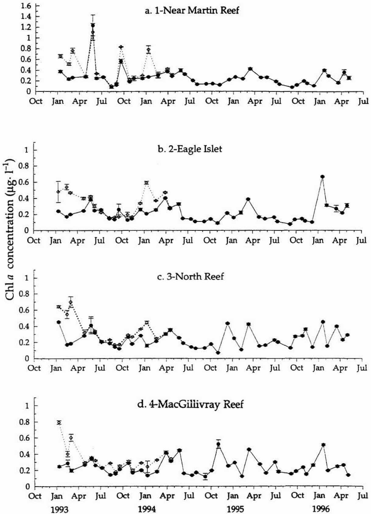
Figure 5.7 Lizard stations 1–4: mean ( \pm 1 S.E.) monthly near-surface ( \bullet ) and near-bottom ( \circ ) chlorophyll a concentrations ( \mu\text{g} \cdot \text{L}^{-1} )
