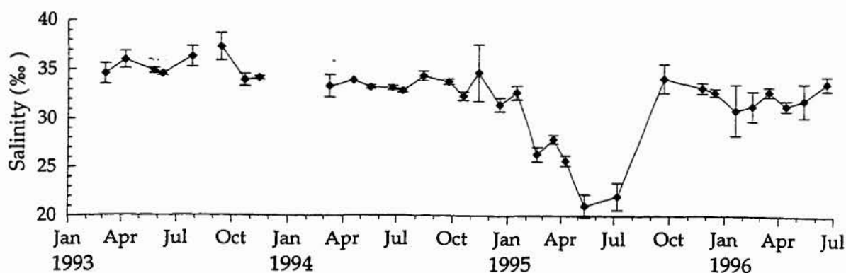
Figure 9.2 Keppel Bay: mean ( \pm 1 S.D.) monthly surface salinity (‰)
