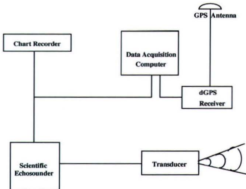
Figure 2. Equipment used in acoustic survey of benthic environments: a) configuration of fan beam transducer when deployed from survey vessel and b) hardware of acoustic systems.
