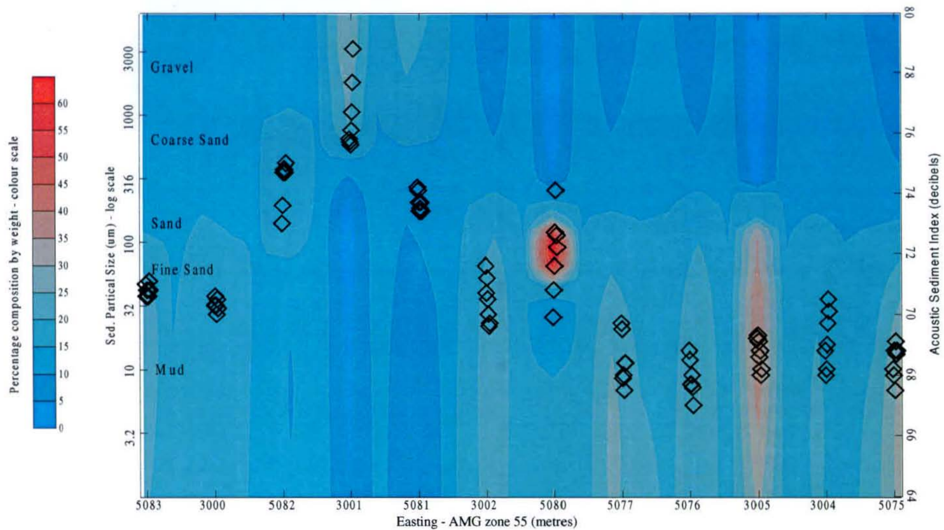
Figure 10. Comparison of acoustic intensity and ground-truthed sediment composition for each sediment sampling site at Bessie Point.
