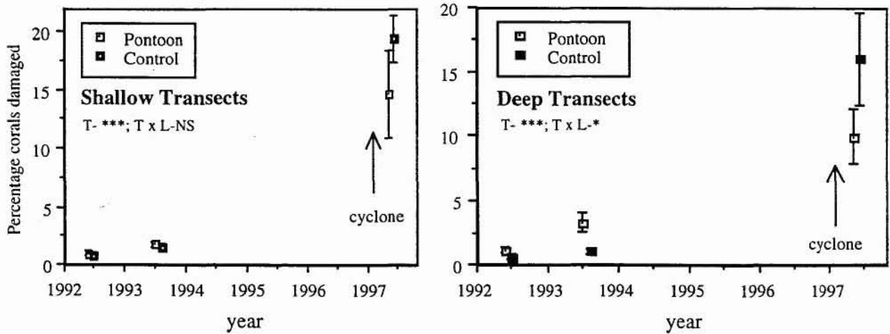
Figure 6. Patterns of coral damage at the pontoon and control locations. Graphs show mean percentage of coral colonies damaged in ten 20 x 1 m transects at each location. The approximate time of the impact from cyclone Justin is indicated. Error bars are standard errors. Significance of tests for time and the time x location interaction are shown. NS = not significant; * = 0.05 > p > 0.01 ; ** = 0.01 > p > 0.001 ; *** = 0.001 > p
