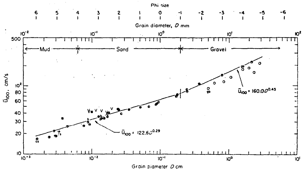
Figure 4: The grain diameter D versus the threshold flow velocity 100 cm above the bed ( U_{100} ) necessary for the movement of quartz density material in water of temperature 20°C. Source: Miller et al. (1977).
