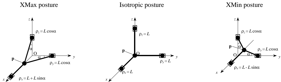
Fig. 4. Specific postures of the Orthoglide manipulator (corresponding to the x-leg leg motion along the Cartesian axis X )
