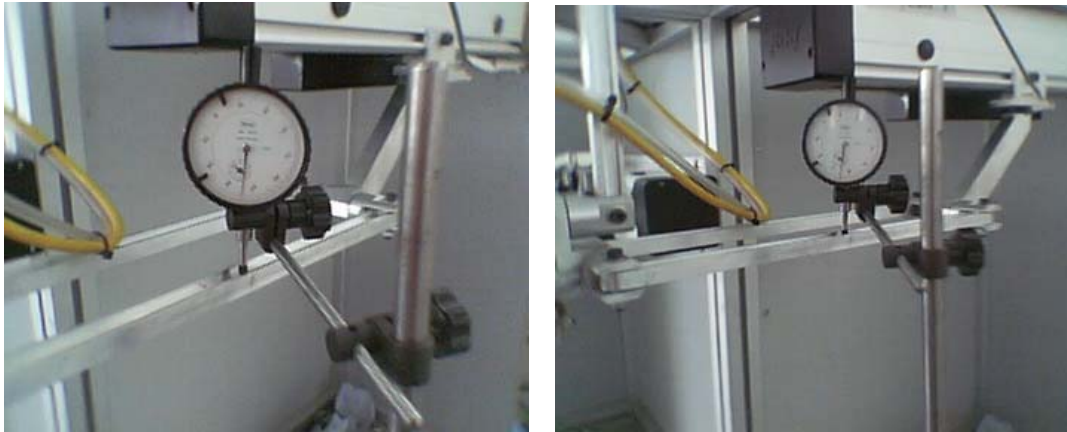
Fig. 6. Experimental Setup.
