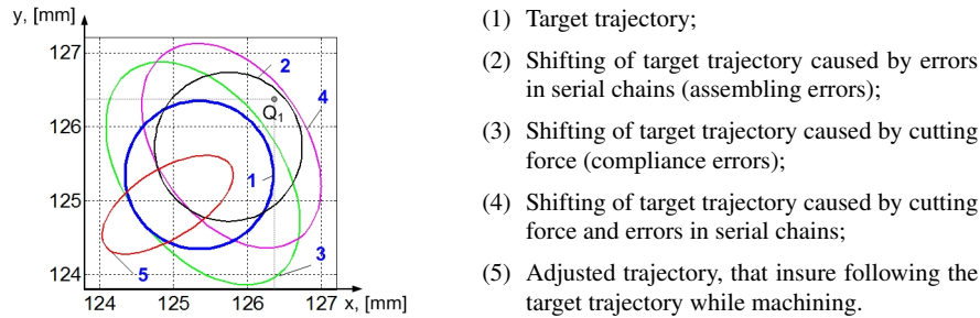
Fig. 4 Influence of different error sources on the machining trajectory.
