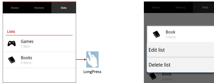
Fig. 3. IFML mobile extension: Example of the LongPress event.
