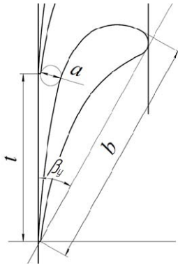
Figure 5. Blade profile TS-1A
