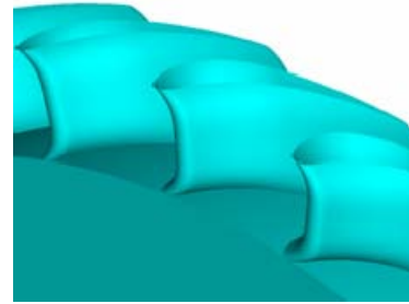
Figure 7. Optimized guide blade rim for a/l=0.22
