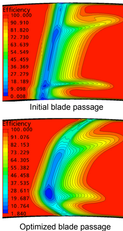
Figure 9. Efficiency field on outlet from blade passage for a/l=0.22
