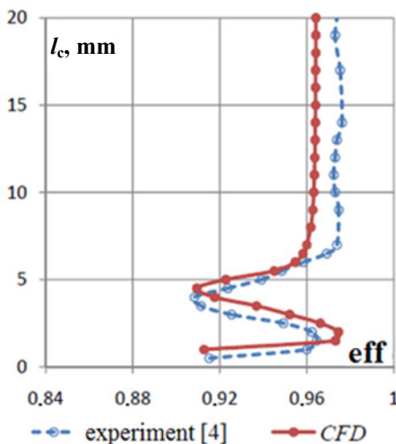
Figure 1. Efficiency distribution along blade height
