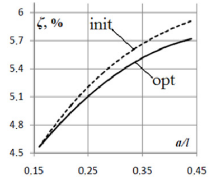
Figure 6. Total losses dependence from a/l and algorithm. The shorter the turbine blade - the more significant gain. On Fig. 7 the optimized guide blade rim is shown at a/l=0.22 .
