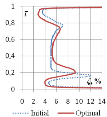
Figure 8. Total loss coefficient distribution along blade passage height
