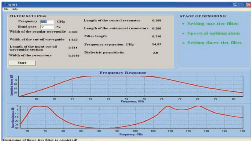
Figure 6b – The comparative characteristic of the frequency response of three-tier 73.5 GHz filter with band pass 7%
