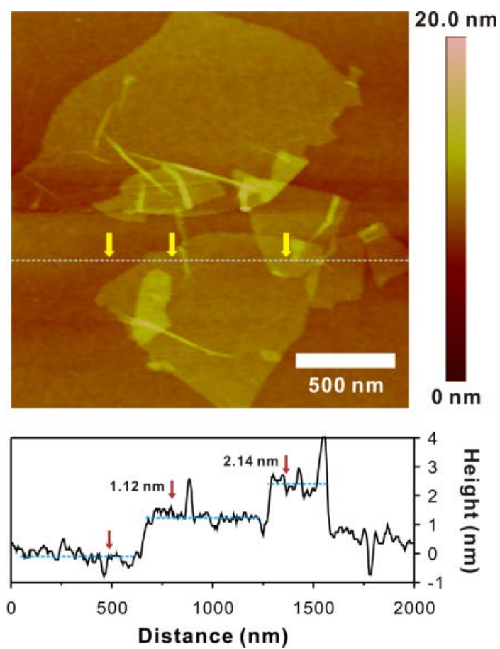
Fig. S2 Representative height-mode AFM images of NGO3 with the corresponding line scan profiles. The height of monolayer and bilayer is about 1.12 nm and 2.14 nm, respectively.
