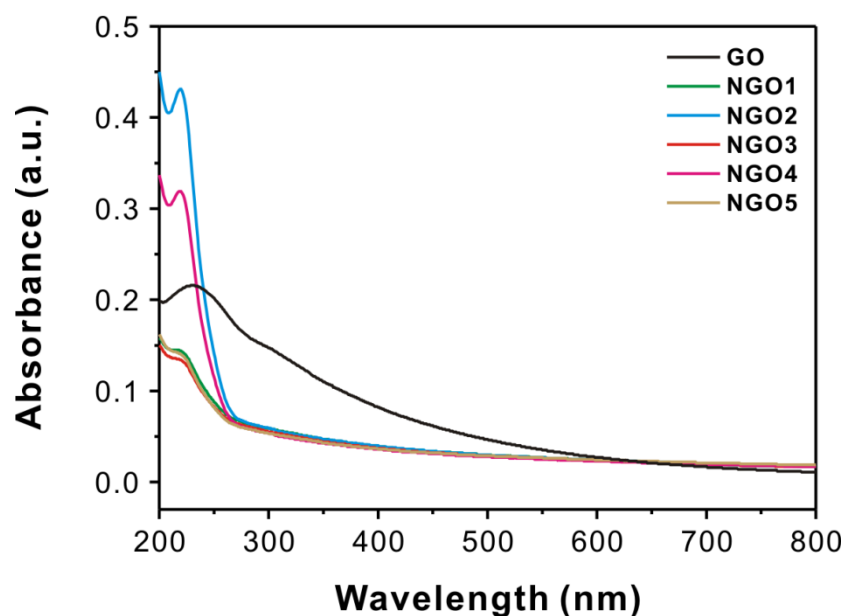
Fig. S1 UV-vis absorbance spectra for GO suspension and NGO n derivatives. Concentration of suspensions is 0.5 \mu\text{g mL}^{-1} .
