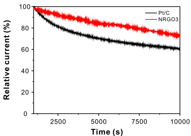
Fig. S4 The chronoamperometric durability response for 10000 s with Pt/C and NRG03.
