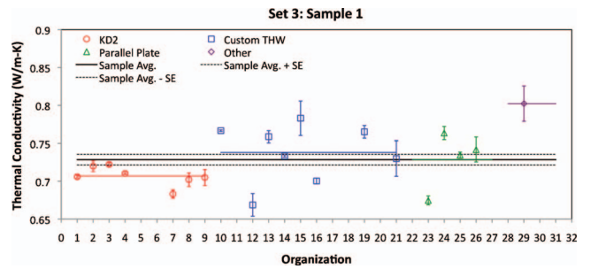
FIG. 15. (Color) Thermal conductivity data for sample 1, set 3.
