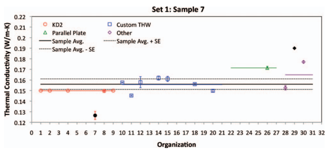
FIG. 12. (Color) Thermal conductivity data for sample 7, set 1.
