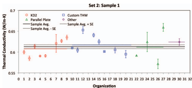
FIG. 13. (Color) Thermal conductivity data for sample 1, set 2.
