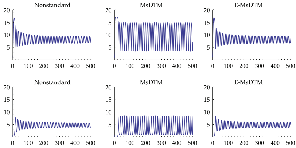
Figure 9: x(t) (Top) and y(t) (Bottom); nonstandard scheme (Left, h = 0.01 ), MsDTM (Middle, h = 0.25 ), E-MsDTM (Right, h = 0.25 ); k = 17.1 .
