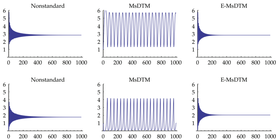
Figure 10: x(t) (Top) and y(t) (Bottom); nonstandard scheme (Left, h = 0.01 ), MsDTM (Middle, h = 0.2 ), E-MsDTM (Right, h = 0.2 ); k = 32\sqrt{2}/7 - 0.1 .
