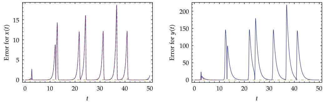
(a) Absolute error with one iteration: x(t) (left), y(t) right
