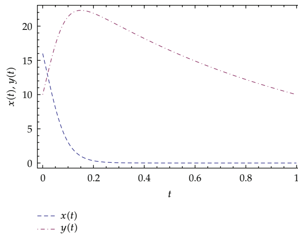
Figure 3: Population of x(t) and y(t) by RK4 ( h = 0.0001 ) in case 2.
