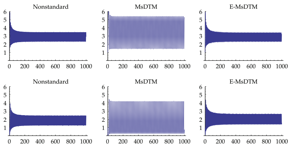
Figure 11: x(t) (Top) and y(t) (Bottom); nonstandard scheme (Left, h = 0.01 ), MsDTM (Middle, h = 0.125 ), E-MsDTM (Right, h = 0.125 ) k = 32\sqrt{2}/7 + 0.1 .
