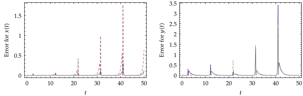
(b) Absolute error with two iterations: x(t) (left), y(t) right
