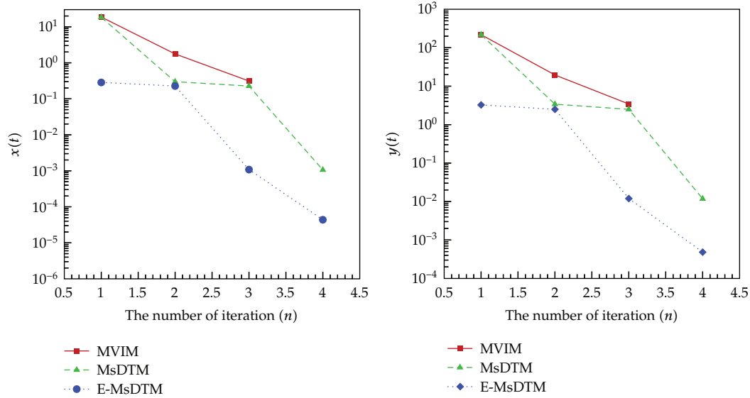
Figure 7: Maximum error with the number of iteration.
