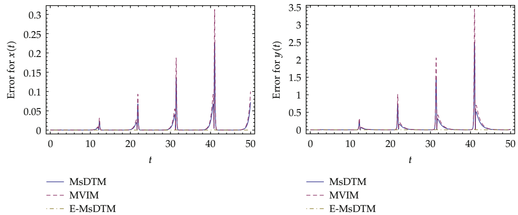
(c) Absolute error with three iterations: x(t) (left), y(t) right
