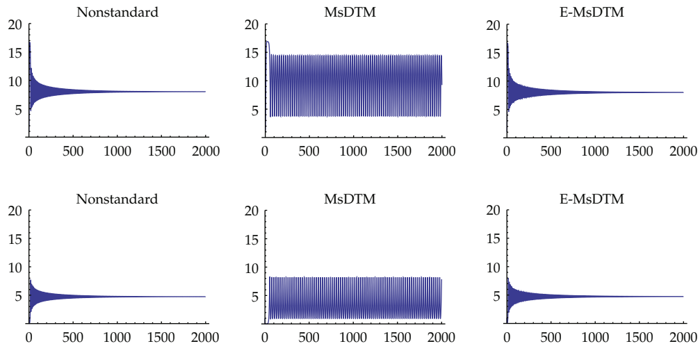
Figure 8: x(t) (Top) and y(t) (Bottom); nonstandard scheme (Left, h = 0.01 ), MsDTM (Middle, h = 0.25 ), E-MsDTM (Right, h = 0.25 ); k = 16.9 .
