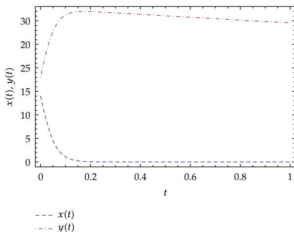
Figure 1: Population of x(t) and y(t) by RK4 ( h = 0.0001 ) in case 1.
