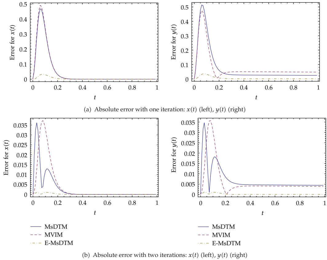
Figure 2: Comparison of absolute errors in case 1.
