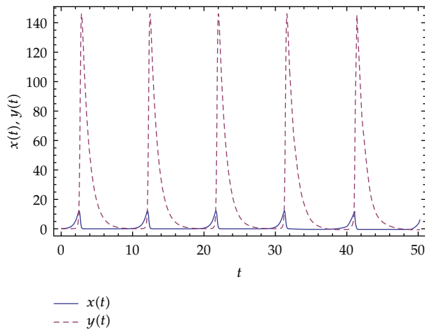
Figure 5: Population of x(t) and y(t) by RK4 ( h = 0.0001 ) in case 3.
