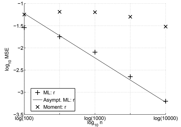
Fig. 2. \log_{10}(\text{MSE}) of \hat{r}_{\text{MV}} versus \log_{10}(n) (10000 MC runs).
