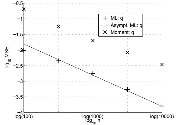
Fig. 1. \log_{10}(\text{MSE}) of \hat{q}_{\text{MV}} versus \log_{10}(n) (10000 MC runs).
