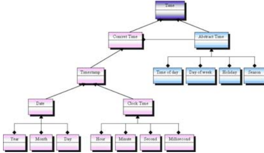
Fig. 2. A simple schema of the time model
