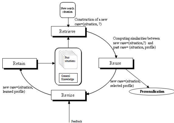
Fig. 3. CBR cycle
