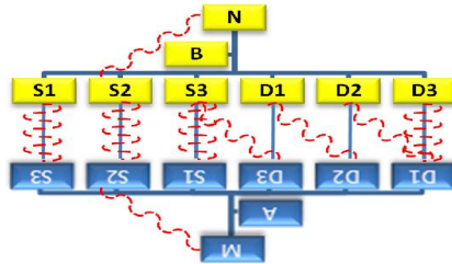
Fig. 1. Inter-organizational model
