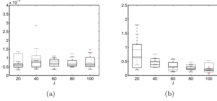
Figure 4: Boxplot of \frac{1}{J}\|\hat{\boldsymbol{\theta}}^\lambda - \boldsymbol{\theta}_{\Theta_0}^*\|^2 (a) and \frac{1}{J}\|\hat{f}^\lambda - f_{\Theta_0}\|^2 (b) in model (3.3) with a stationary error term Z . Boxplot in gray correspond to n = 512 , and in black to n = 1024 .
