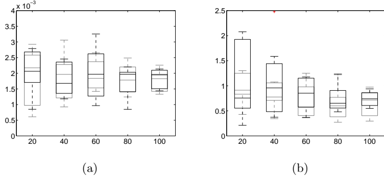
Figure 5: Boxplot of \frac{1}{J}\|\hat{\boldsymbol{\theta}}^\lambda - \boldsymbol{\theta}_{\Theta_0}^*\|^2 (a) and \frac{1}{J}\|\hat{f}^\lambda - f_{\Theta_0}\|^2 (b) in model (3.3) with a non-stationary error term Z . Boxplot in gray correspond to n = 512 , and in black to n = 1024 .
