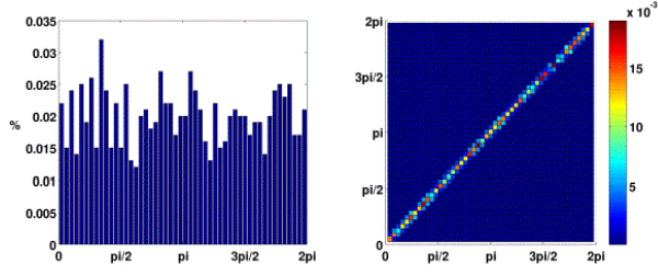
(a) N = 10^2
