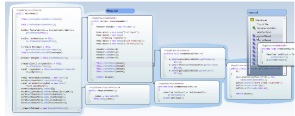
Figure 11. Code Bubble classification.
