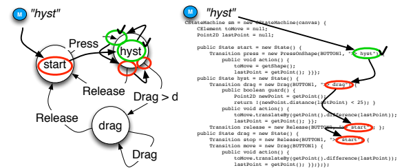
Figure 17. ScanVis for the task: “what are the in transitions for state ‘hyst’?”
