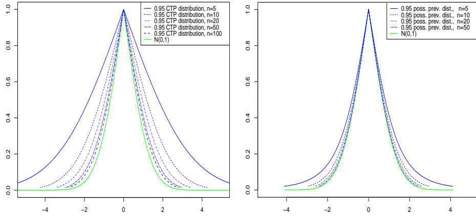
Fig. 4. 0.95-confidence tolerance possibility distribution for different sample sizes having (\bar{X}, S) = (0, 1) . Fig. 5. 0.95-confidence prevision possibility distribution for different sample sizes having (\bar{X}, S) = (0, 1) .
