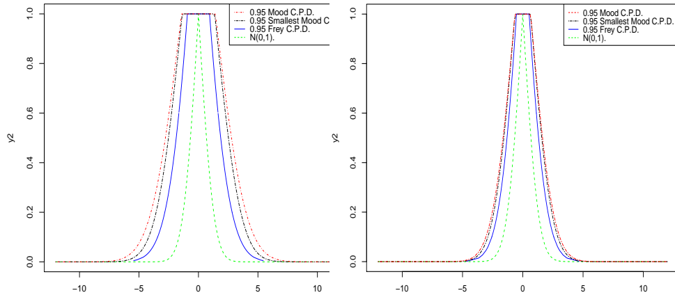
Fig. 2. Possibility distribution encoding normal confidence band for a sample set of size 10 having (\bar{X}, S) = (0, 1) . Fig. 3. Possibility distribution encoding normal confidence band for a sample set of size 25 having (\bar{X}, S) = (0, 1) .
