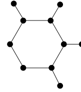
Fig. 3: The consecutive broken sun CBSun_{6,4}
