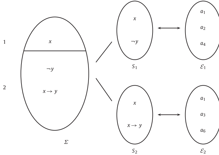
Fig. 1. Preferred sub-theories of \Sigma vs. stable extensions of (\text{Arg}(\Sigma), \text{Undercut}, \succeq_{\text{WLP}}) .
