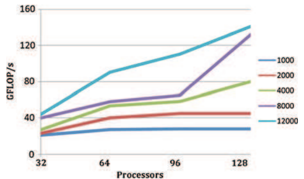
Fig. 5 ScaLAPACK PDGEMM benchmarking on Armcluster (performance in GFlops vs number of processors)
