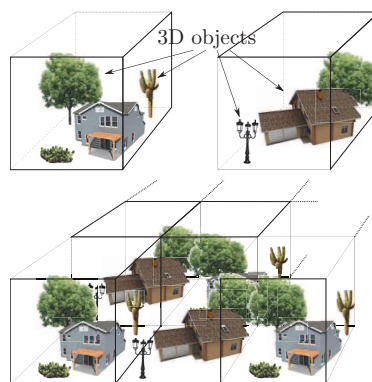
Figure 1: Using a tiling set of two predefined tiles (top) in a 3D world tiling process (bottom). Objects are placed into these tiles forming the tiling set. These are randomly or deterministically instantiated in 3D space to form the final world geometry.
