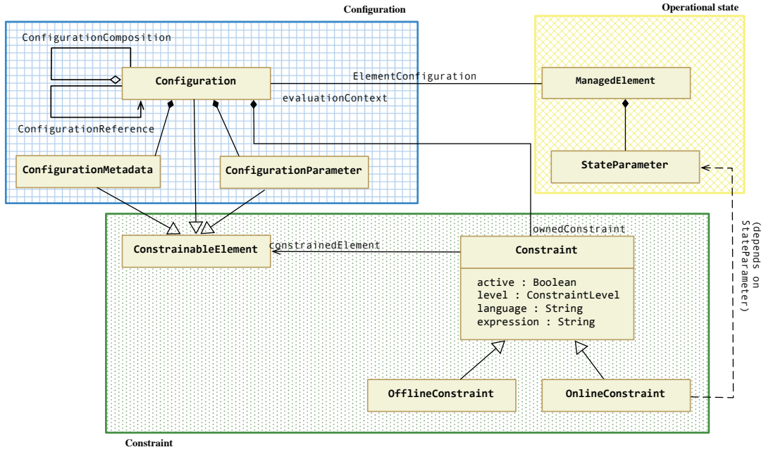
Fig. 5. Overview of the MeCSV metamodel
