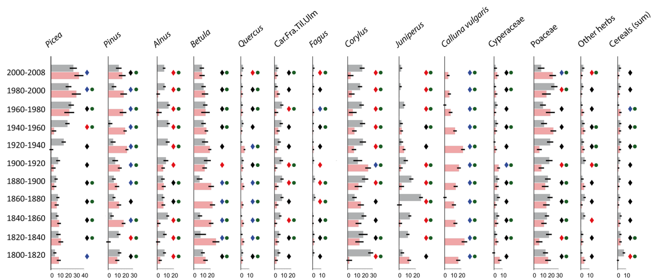
Fig. 7 LRA-inferred local vegetation compositions based on 14 taxa for Abodasjön ( grey ) and Lindhultsgöl ( pink ) compared with the output of the QAD method. The QAD results are indicated by solid diamonds on the right-hand side of each taxon. The colour code for
