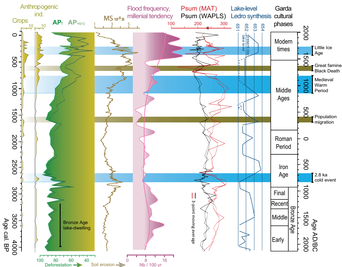
Figure 6. Ledro's record of agricultural activities, forest cover (arboreal pollen, inversed scale), erosion in the catchment (MS), flood frequency (Vannièr et al., 2013), lake levels (Magny et al., 2012), and pollen-based reconstructed summer precipitation (the star indicates the present-day summer precipitation; Peyron et al., 2013). Climatically and non-climatically induced vegetation and land-use changes are shown in blue and brown, respectively.
