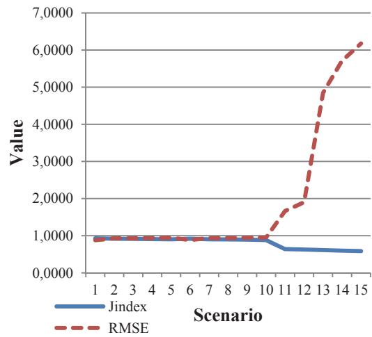
Figure 3: RMSE & Jaccard index on whole data sets.
