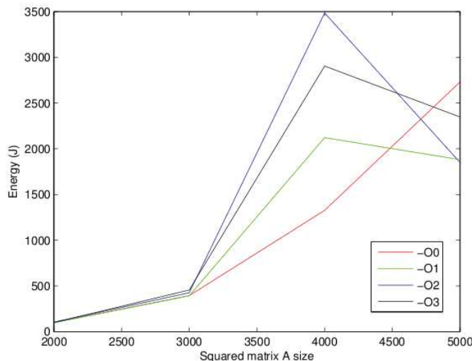
Figure 3. Energy dissipated to solve a linear system of equations using LAPACK
