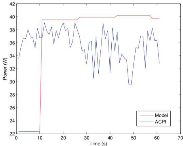
Figure 2. Comparison between ACPI power meter and the linear model
