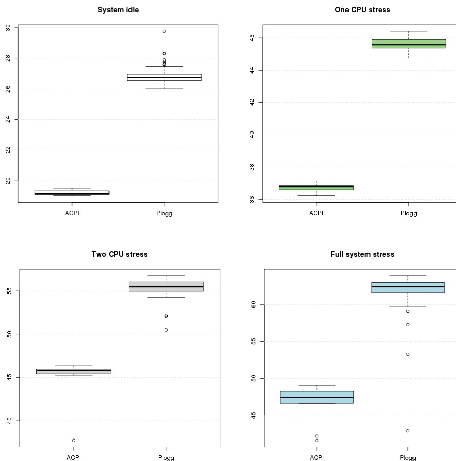
Figure 1. Comparison between ACPI and Plogg power meters for distinct workloads
