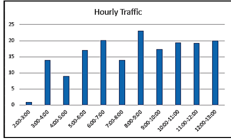
Fig. 4. Outcome from the simulation model using the trailing set as data sample
