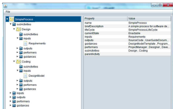
Figure 12: Example of collaborative simple process.
