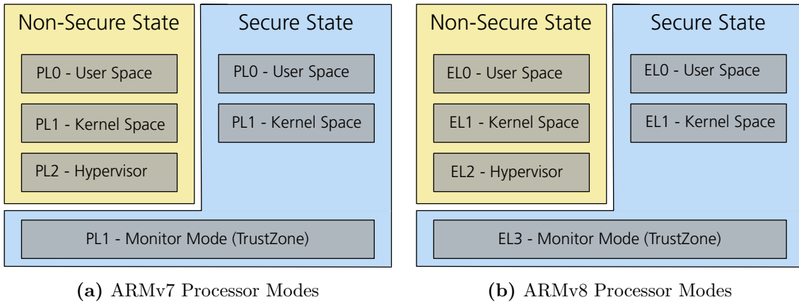
Figure 2.6: Difference between processor modes in ARMv7 (Privilege Levels) and ARMv8 (Exception Levels)
