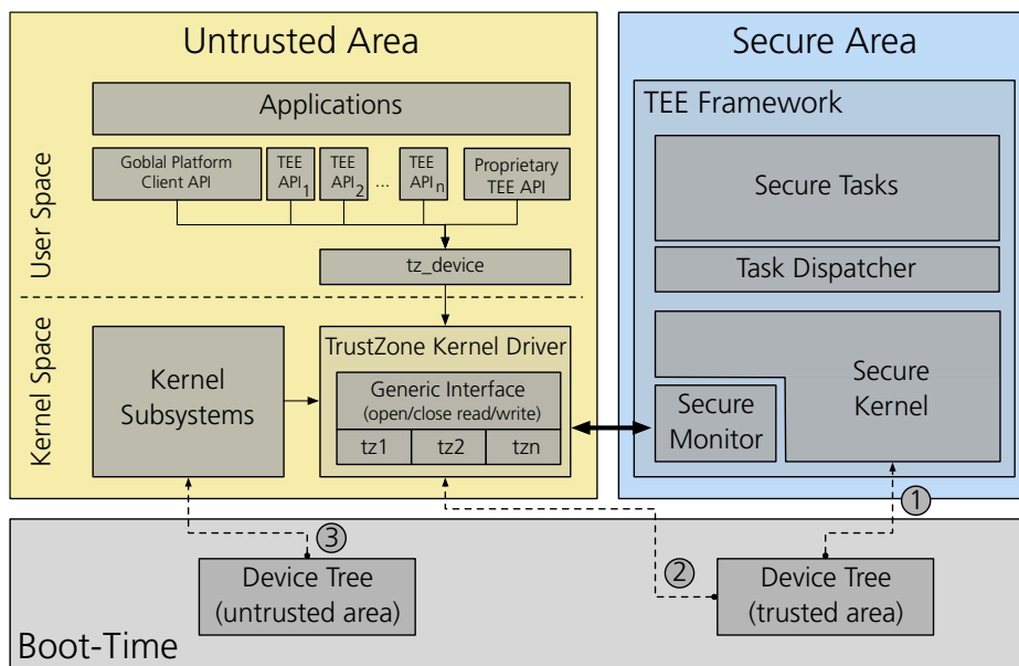
Figure 7.1: Generic TrustZone Driver Architecture. Boot-time information is included to depict the concept of the Secure Device Tree which corresponds to Device Tree (trusted area).
