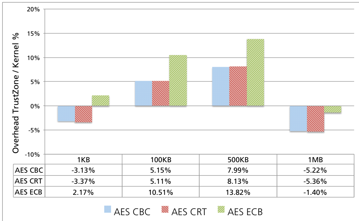
Figure 11.6: Encryption overhead of using the AES algorithm with a 128-bit key and different block ciphers modes. Kernel space relies on Linux Kernel crypto API; secure space uses the libcrypto EVP API available in OpenSSL.
