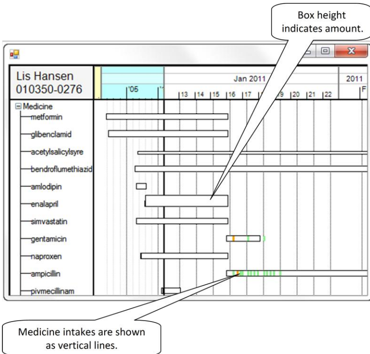
Figure 10 - An example of advanced visualizations developed in VisTool
