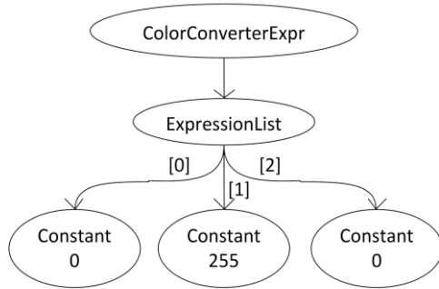
Figure 43 - Color converter for an integer array
