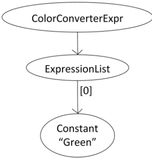
Figure 42 - Color converter for string
