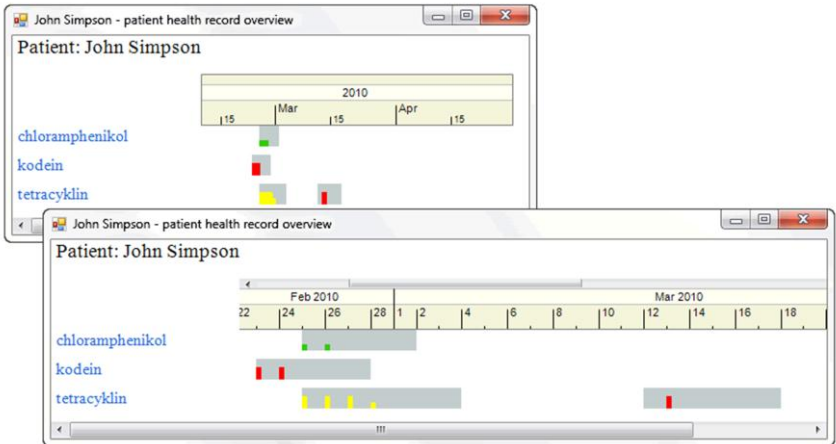
Figure 35 - Change the timescale zooming factor
