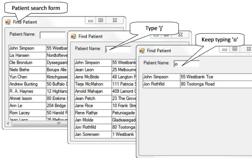
Figure 39 - The patient-search form
