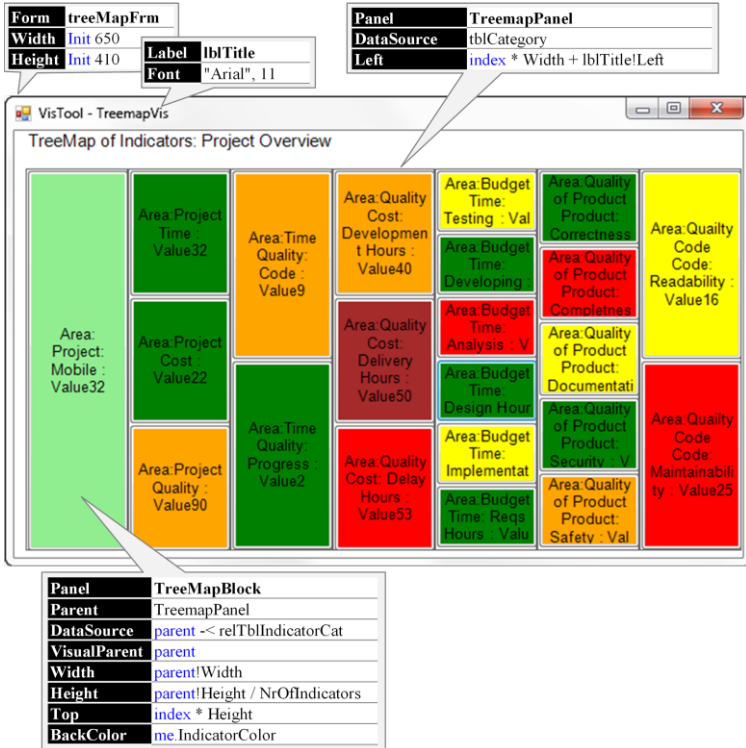
Figure 57 - TreemapVis' templates and formulas
