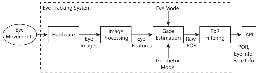
Figure 3.4: A model of a VOG eye tracking system. Eye movements are recorded and manipulated by several stages until the point-of-regard and tracking related information are delivered to the API. Everything within the dashed line is essentially a ‘black box’ but the individual stages and their functionality can to some extent be guessed.
