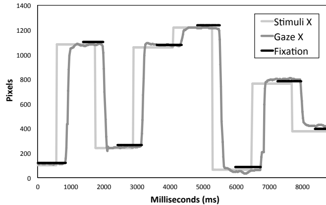
Figure 3.7: Eight stimuli (light grey) and the resulting gaze signal (dark grey) recorded with an Eye Follower from LC Technologies running at 60 Hz for each eye, offset for 120 Hz frame rate. This system allows access to the raw data. Here, corresponding fixations (black) in the gaze signal have been detected by a hybrid fixation-detection algorithm designed for investigative purposes by the author, bypassing the system’s own event detection algorithm.
