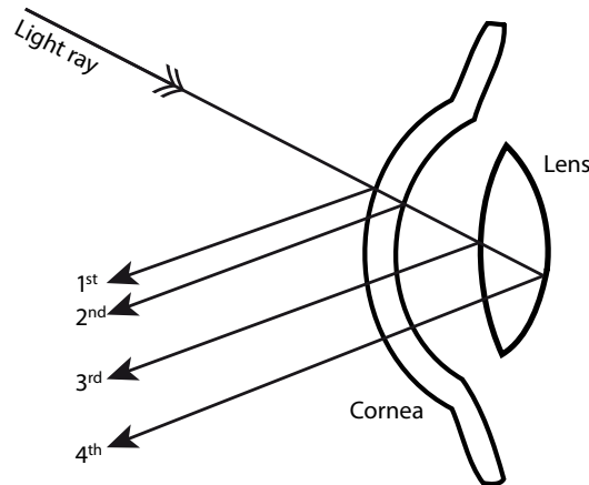
Figure 2.2: Arrangement of the four Purkinje images. Adapted from the Fourward Technologies, Inc. < http://www.fourward.com >.
