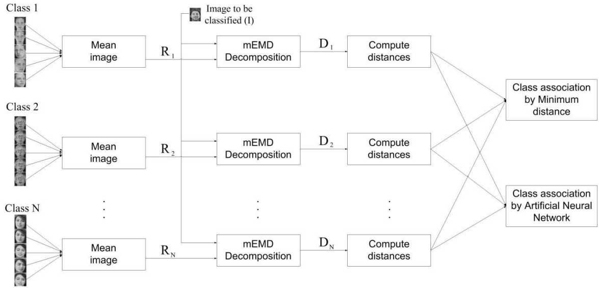
Figure 2: Scheme of the proposed image processing procedure.
