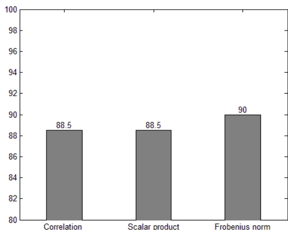
Figure 3: Obtained classification rates (%) for the three different distances using the first method: class association only based on the criterion of minimum distance. Exact experimental values are presented at the top of each bar.
