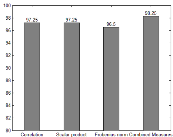
Figure 4: Obtained classification rates (%) for the three different distances and the combination of all of them, using the second method: an ANN as a classifier. Exact experimental values are presented at the top of each bar.
