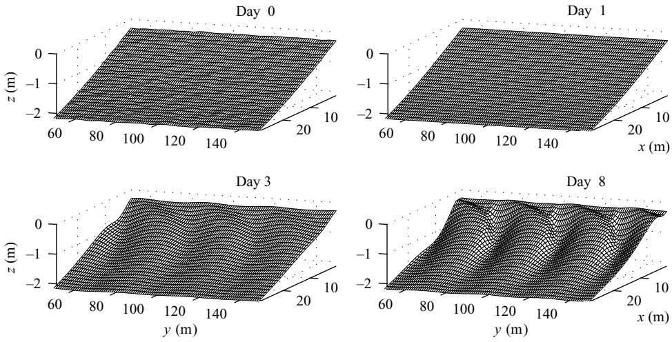
FIGURE 7. SVR transport, H_{rms} = 1.0 m, T = 6 s, \theta = 25^\circ . Zoom of the total bathymetry during the formation, development and growth saturation of oblique down-current oriented bars.
