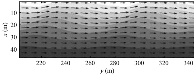
FIGURE 11. CWS transport, H_{rms} = 1.0 m, T = 6 s, \theta = 25^\circ . Final state (day 85). Bathymetric contours ( z_b ) and circulation ( \mathbf{v} ) over up-current oriented bars. Shallowest areas are white and deepest areas are shaded.
