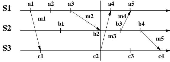
Figure 3: Event-driven Causality
