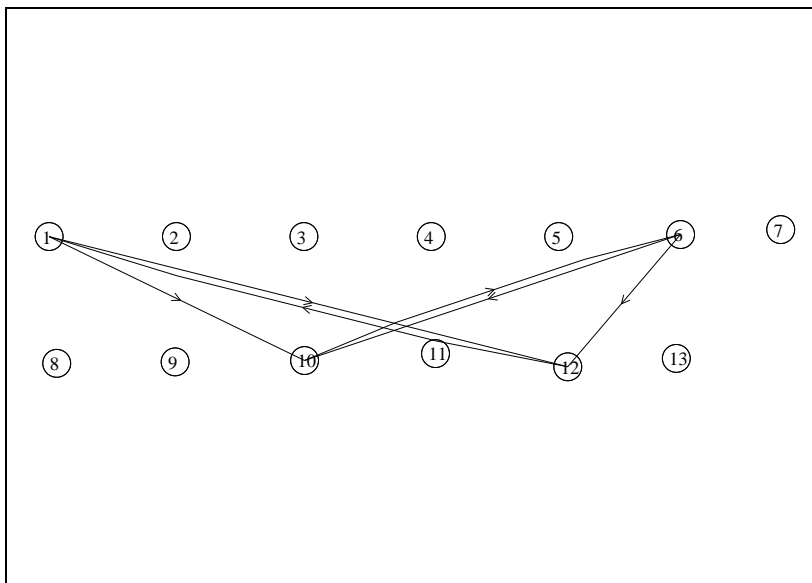
Figure 7: Graph G1
