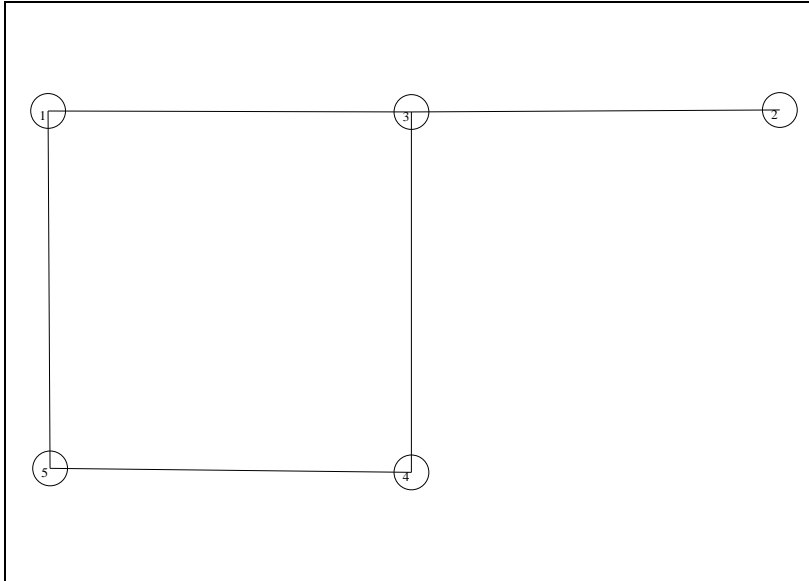
Figure 1: Adjacency structure
