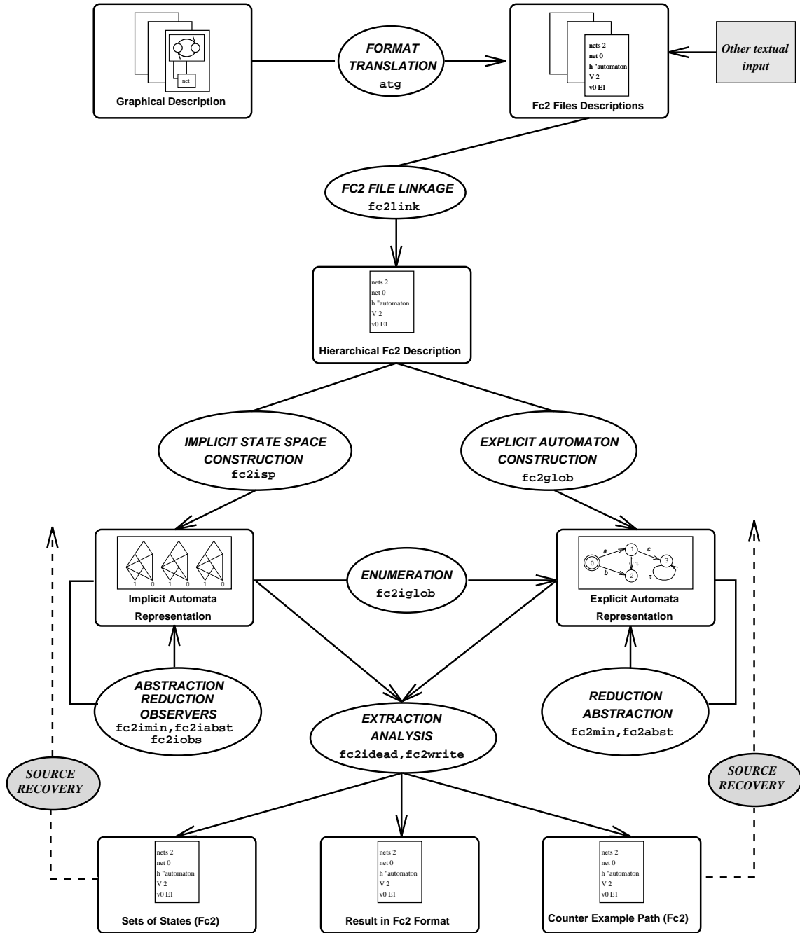
Figure 1: Software hierarchy
