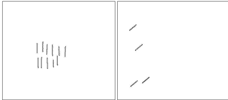
Figure 8: Grouping in the space (x\text{-coordinate,orientation}) . There are two maximal meaningful groups. This time, the whole central group is detected ( NFA_g = 10^{-1.5} ), but there is still another group (which is a part of the 7th group in the orientation grouping (see Fig. 7)). However, its NFA_g = 0.3 , which means that it is hardly meaningful. If grouping is done with respect to full 2D-position and orientation, only the central group is detected with NFA_g = 10^{-3.4} .
