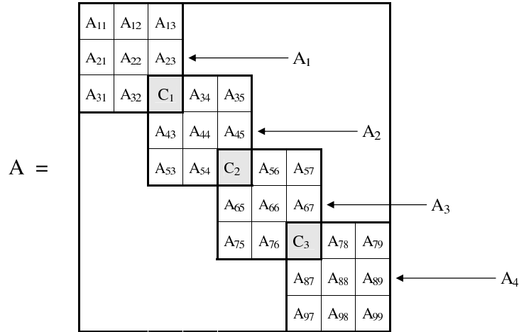
Figure 1: A matrix domain decomposition with block overlaps. W_1 = w_1 \cup w_2 \cup w_3 , W_2 = w_3 \cup w_4 \cup w_5 , W_3 = w_5 \cup w_6 \cup w_7 , W_4 = w_7 \cup w_8 \cup w_9 , where, for i = 1, \dots, 9 , w_i is the set of the row indices of A_{ii} with C_1 = A_{33} , C_2 = A_{55} and C_3 = A_{77} .
