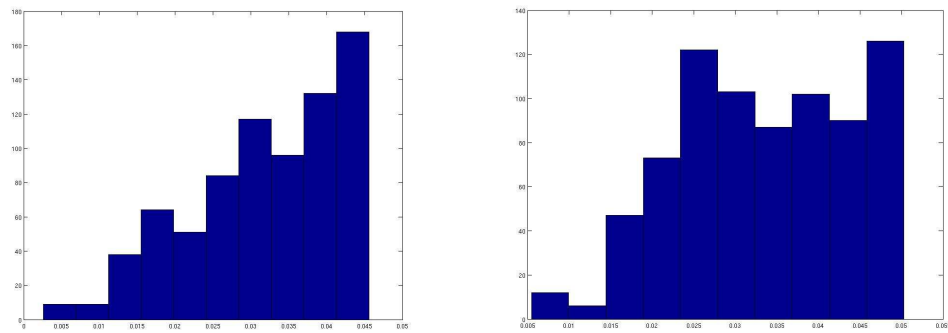
Figure 4: Dense extrapolation of tensors with harmonic diffusion: comparison of anisotropy. Left: histogram of the relative difference (i.e. the difference divided by the first term) between the fractional anisotropy of the Log-Euclidean extrapolation and its affine-invariant counterpart. Right: histogram of the relative difference between the largest eigenvalue of the Log-Euclidean extrapolation and its affine-invariant counterpart. Note that the differences are always positive: the anisotropy is larger in the Log-Euclidean case.
