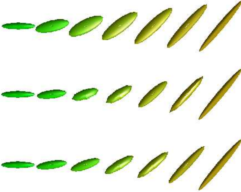
Figure 1: Linear interpolation of two tensors. Above: linear interpolation on coefficients. Middle: affine-invariant interpolation. Below: Log-Euclidean interpolation. Note the characteristic swelling effect observed in the Euclidean case, which is not present in both Riemannian frameworks. Note also that Log-Euclidean means are more anisotropic their affine-invariant counterparts.
