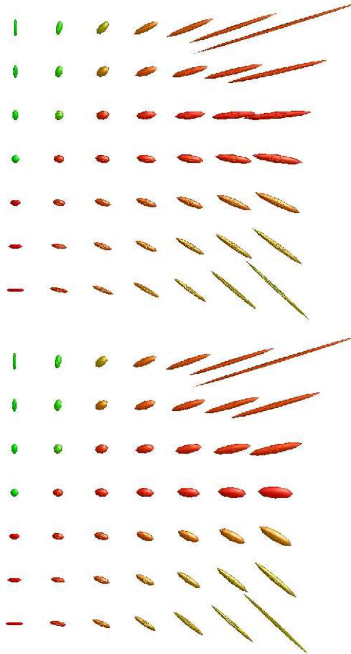
Figure 2: Bilinear interpolation of four tensors. Above: Log-Euclidean mean. Below: affine-invariant mean. Notice that the interpolation is the same to the left along the first column, because the two interpolated tensors commute. On the contrary, results are substantially different on the right: as expected, the anisotropy is larger in the Log-Euclidean case.
