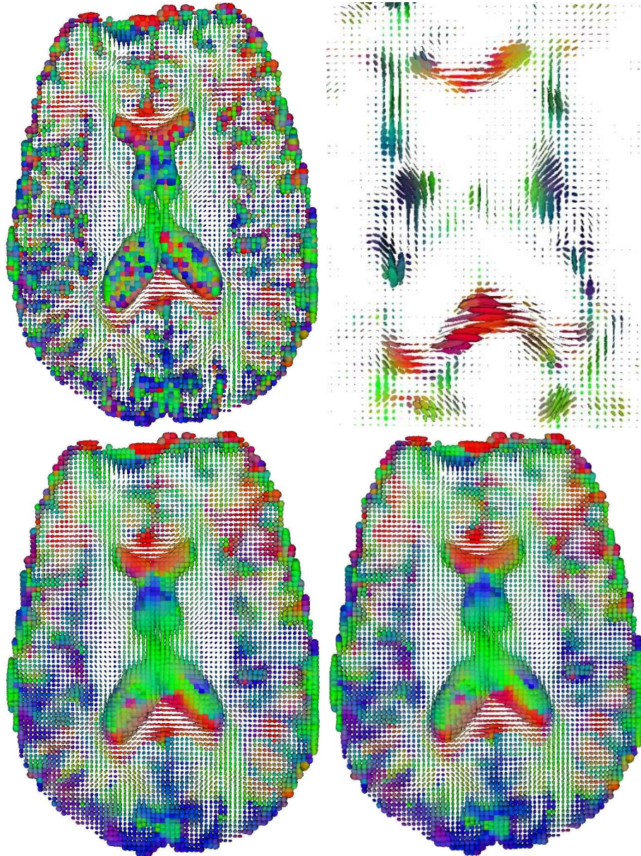
Figure 5: Anisotropic filtering of a DTI slice. Upper Left: raw DTI slice. Upper Right: zoom on a highly magnified visualization of the absolute value of the Euclidean differences between the two results (magnification factor of approximately 1000). Lower Left: affine-invariant result. Lower Right: Log-Euclidean result. Note that the differences are very small, and are concentrated along the directions of anisotropy. Note that there is no tensor swelling whatsoever, contrary to the Euclidean case.
