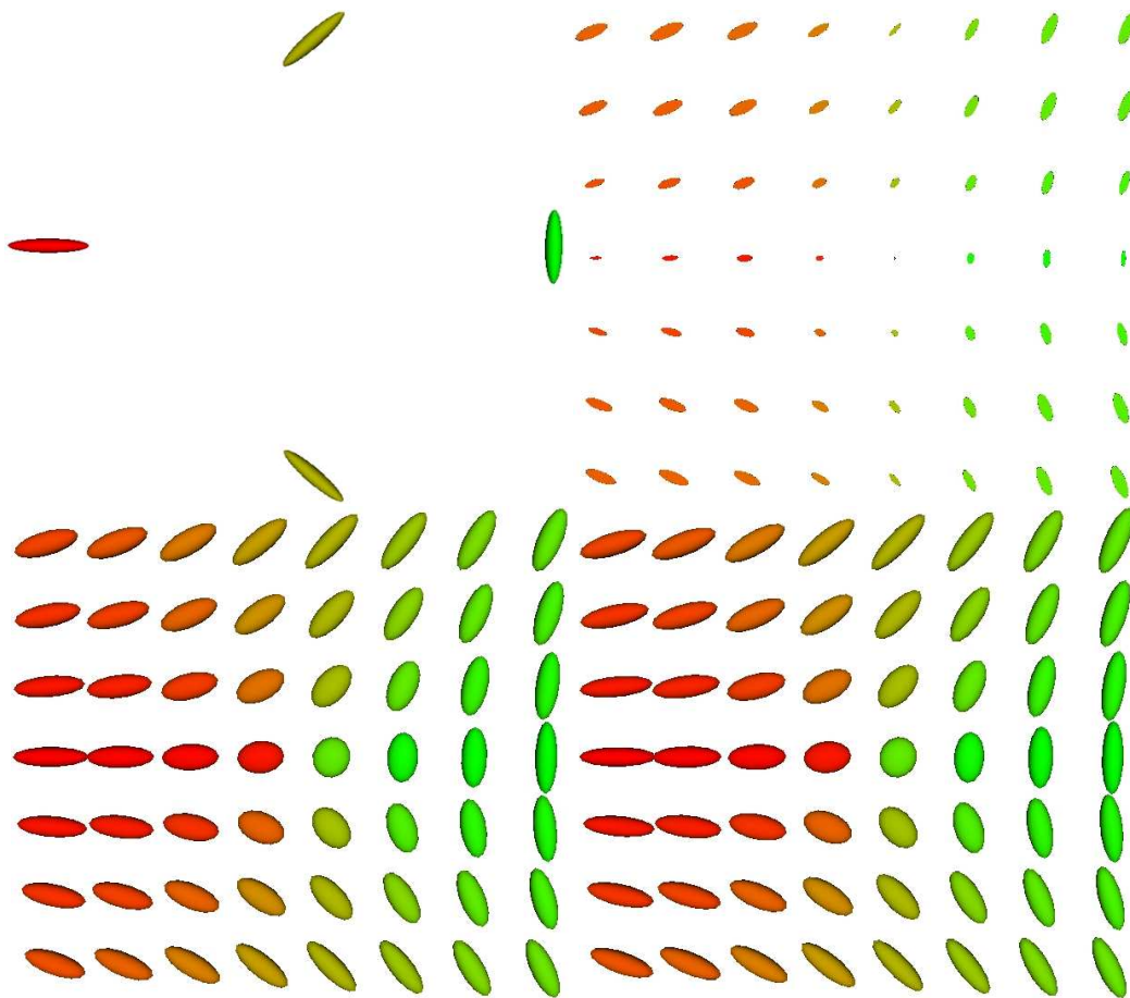
Figure 3: Dense extrapolation of tensors with harmonic diffusion. Upper Left: germs. Upper Right: magnified visualization of the absolute value of the Euclidean difference between the two extrapolations. Lower Left: affine-invariant extrapolation. Lower Right: Log-Euclidean extrapolation. Note that the Log-Euclidean extrapolation yields tensors a little more anisotropic. The differences are very small, and are mostly concentrated along the direction of anisotropy.
