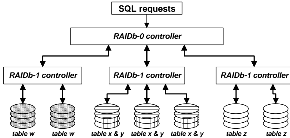
Figure 7. Example of a RAIDb-0-1 composition
