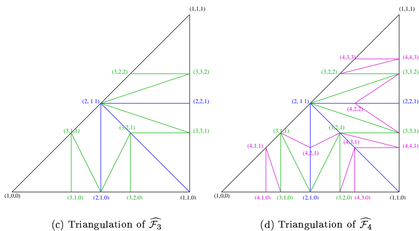
Figure 31: Projection of Farey Triangulation on the plan x = 1
