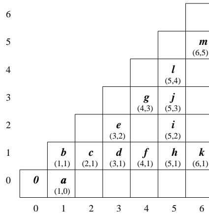
Figure 29: first 2D visible points
