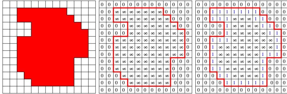
(a) initial object (b) initialization (0 & infinity) (c) border pixels
