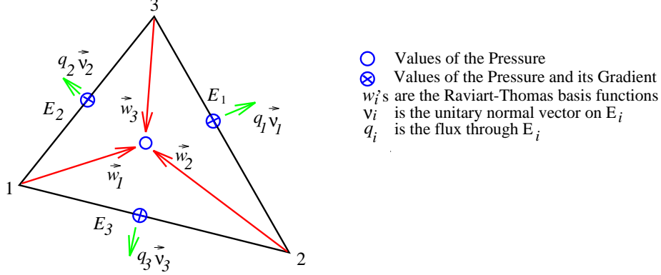
Figure 1: Nodal points and basis functions on triangular elements.
