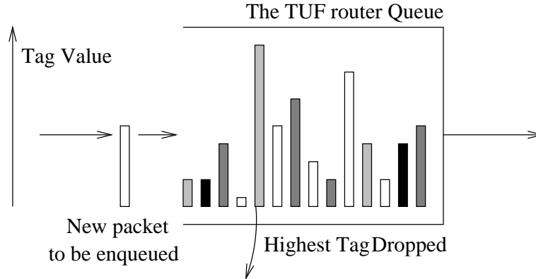
Figure 3: The queueing discipline in a \mathcal{TUF} router
