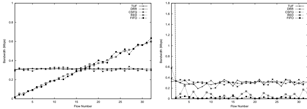
Figure 9: Throughputs for N=32 flows sharing the same 10 Mbps bottleneck link. (a)The arrival rate for UDP flow (i=0..32) is (i+1) times the fair share rate. (b)The UDP flow (ID=0) is sending at 10 Mbps shares the link with 31 other TCP flows.
