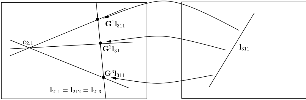
Figure 10: The three lines l_{21i} , i = 1, 2, 3 are identical, see the proof of proposition 25.
