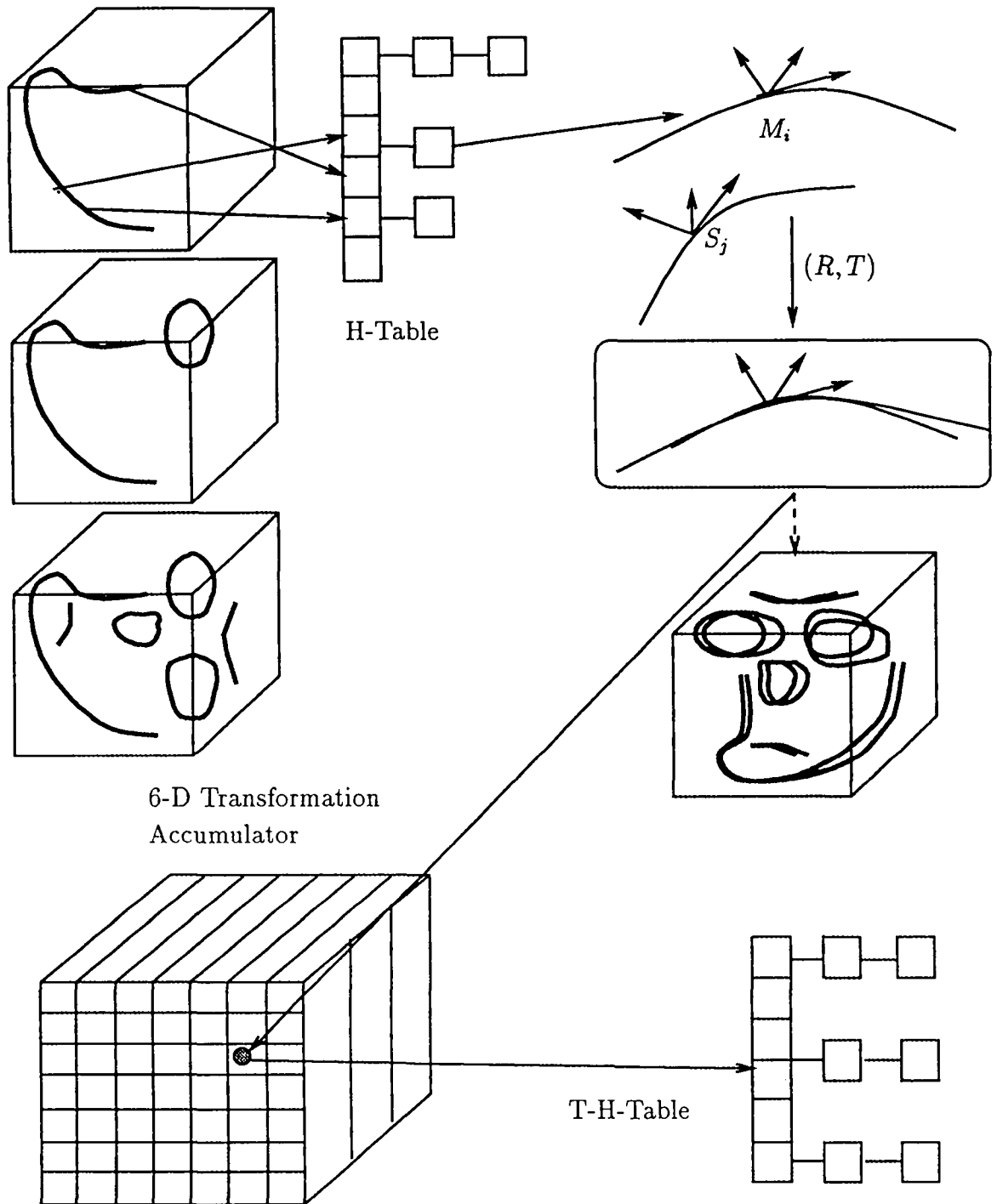
Figure 14: Recognition: each time a 29 ridge point of the scene is matched with a model point through the previous hash table, the Frenet frames allow the computation of the 6 parameters of a rigid displacement (R, t) . This displacement is stored in a 6 dimension accumulator, which is stored with another Hash table. (Courtesy of A. Guézic).
