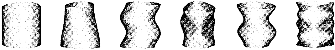
Figure 22: Energy-increasing vibration modes of a cylinder
