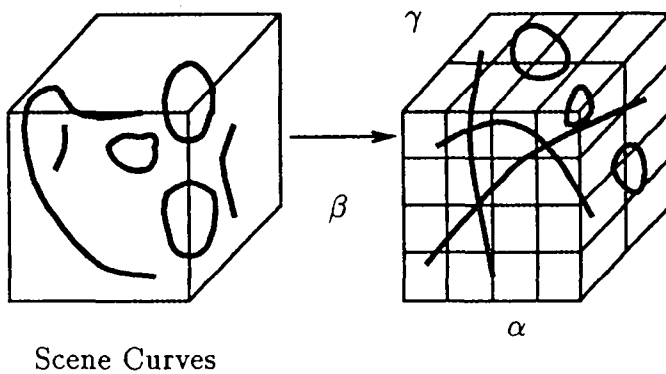
Figure 13: Preprocessing: each ridge point of the model, is stored in a hash table of dimension 5, after the computation of 5 independent intrinsic parameters. At recognition time, the same ridge point, although in another position and orientation, will point towards the same cell of the hash table. (Courtesy of A. Guézic).
